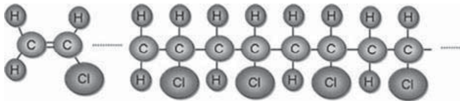
Fig. 2: Vinyl chloride and isotactic PVC (Baudrit 2007)
