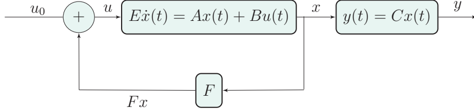
Figure 2.2: Sketch of a state-feedback loop.
