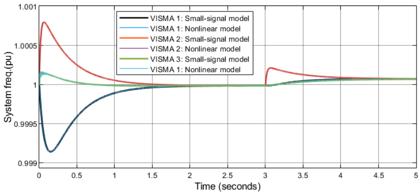
Figure 5.7. Comparing step response in frequency (pu) for both NL and LS models due to step change in input torque
