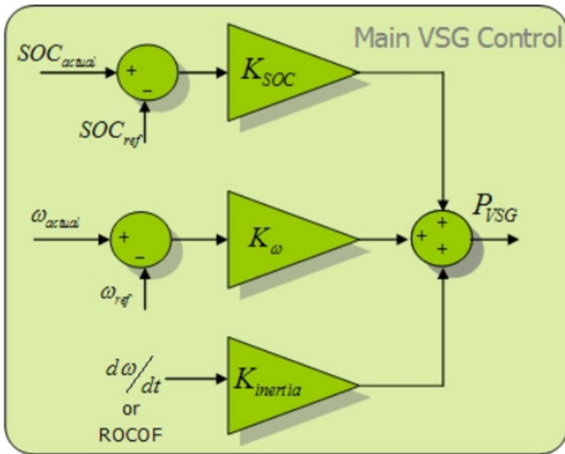
Figure 2.16. VSYNC (a) complete configuration model (b) Main VSG control block [67]
