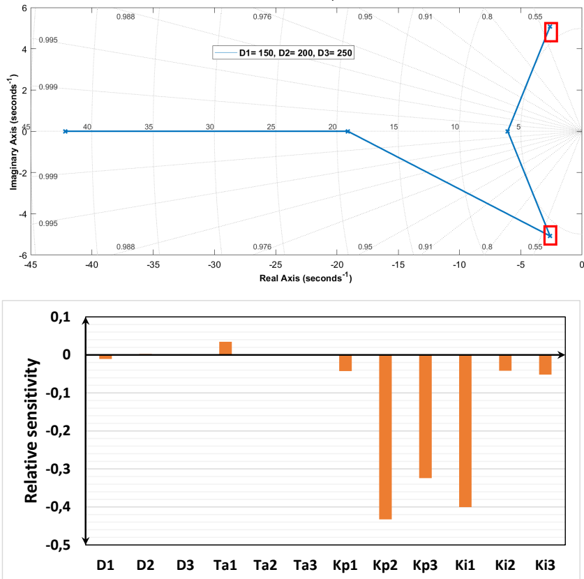
Figure 6. 5. Parameter sensitivity of the Dominant system pole (Case 3).
