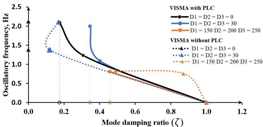
Figure 6.3. Impact of damping on system pole locations.
