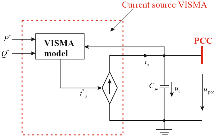
Figure 2.7. Single-phase current control with a two-position controller [29]
