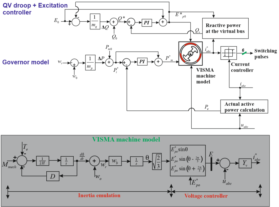
Figure 6.1. VISMA model with control.
