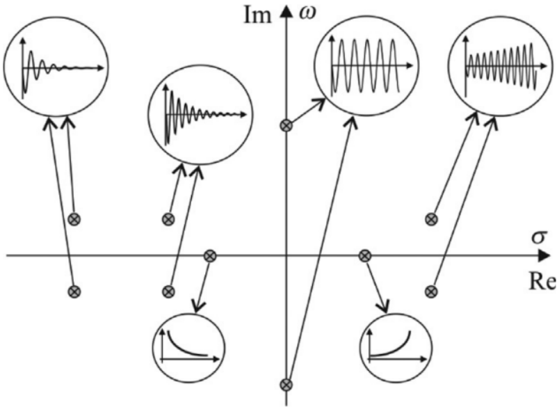
Figure 3.2. Mode type description on the complex plane [27]
