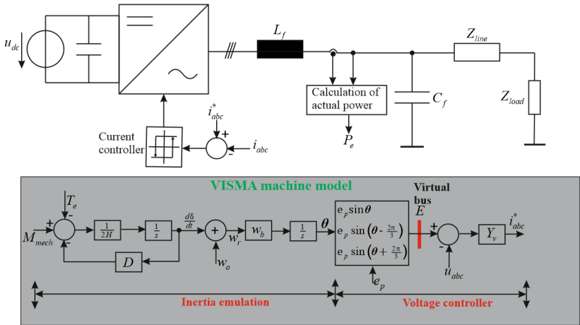
Figure 4.2. Block diagram representation of VISMA
