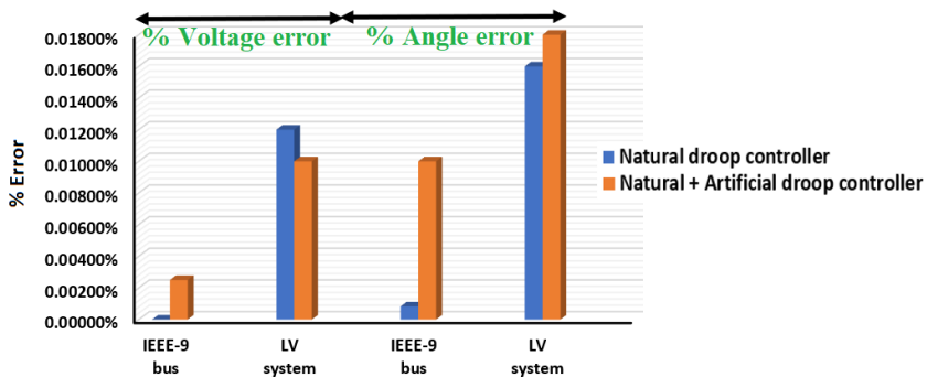
Figure 4.13. Comparative percentage error between LV & HV systems
