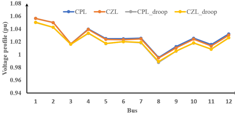
Figure 4.7. Voltage profile for different load type and control
