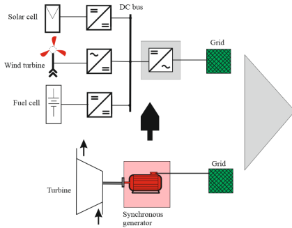
Figure 1.6. Basic structure of VISMA [18]
