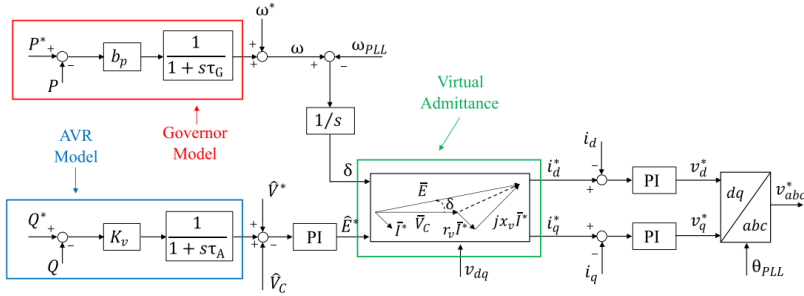
Figure 2.17. KHI control scheme [29]
