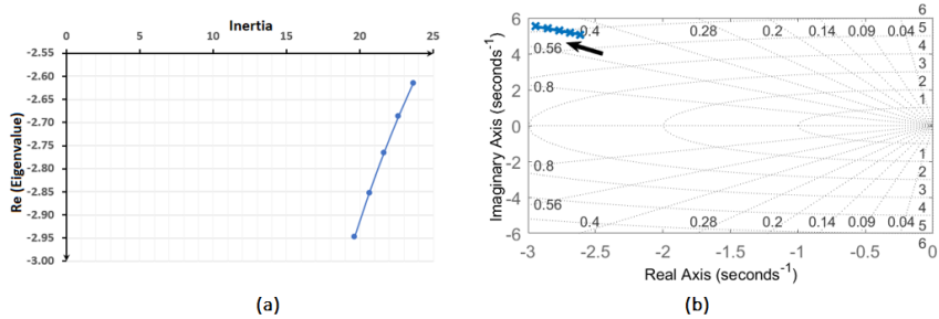
Figure 6.7. Effect of reduced inertia on the dominant mode (a) Inertia Vs real (Eigenvalue) (b) eigenvalue trajectory
