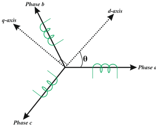
Figure 2.11. 3 – \phi machine and d-q equivalent
