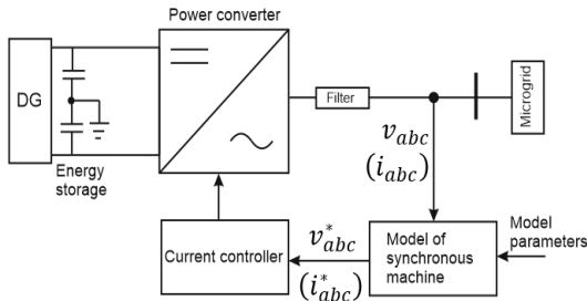
Figure 2.2. Simplified VISMA configuration based on current–voltage (voltage–current) model of
