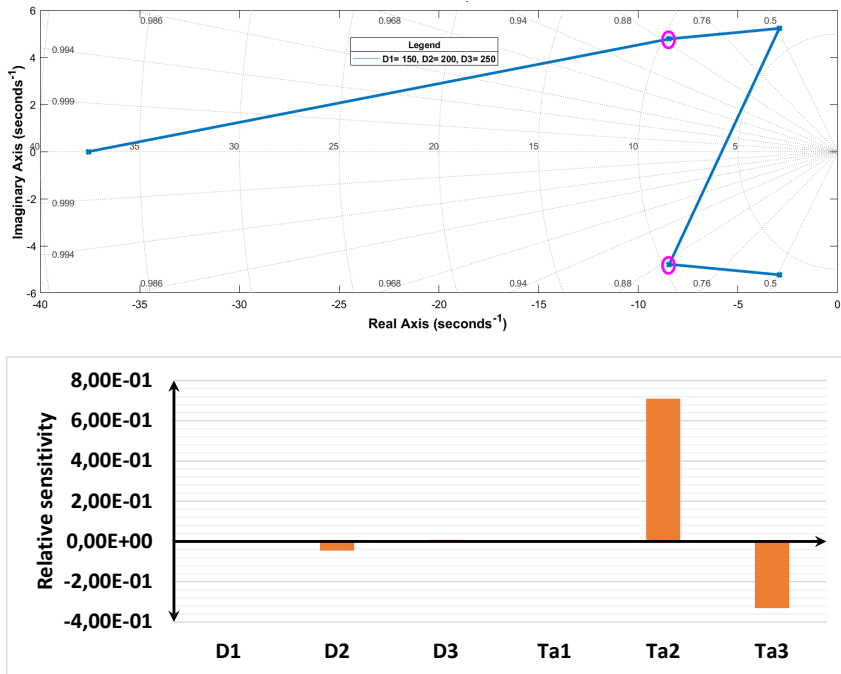
Figure 5.13. Parameter sensitivity of the fastest oscillatory mode
