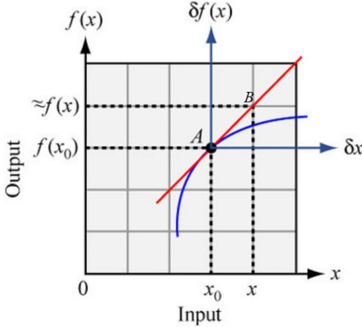
Figure 3.1. Illustrative example of linearization in dynamical systems [135]
