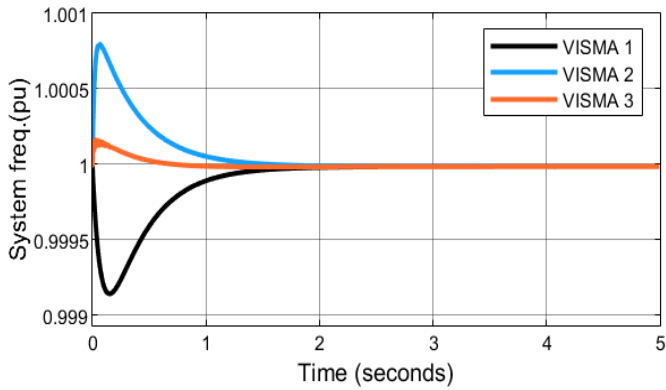
Figure 4.8. System frequency
