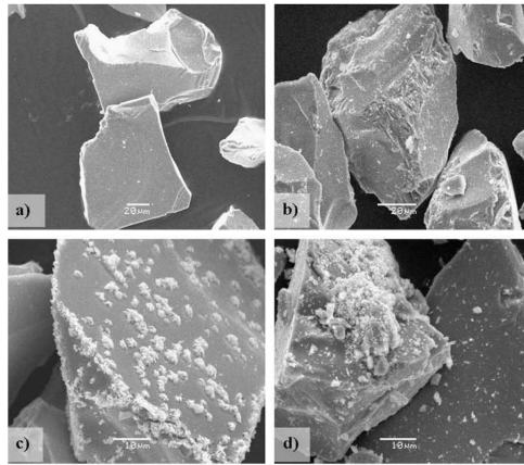
Figure 2.17: Scanning electron microscope (SEM) images of pyrite-to-pyrrhotite reduction observed in Truche et al. [150] - a) pure pyrite sample ( 40 \mu\text{m} to 80 \mu\text{m} sized); partially reacted pyrite after 300 hrs: b) 90^\circ\text{C} , p_{\text{H}_2} = 8 \text{ bar} ; c) 150^\circ\text{C} , p_{\text{H}_2} = 8 \text{ bar} ; d) 150^\circ\text{C} , p_{\text{H}_2} = 15 \text{ bar}
