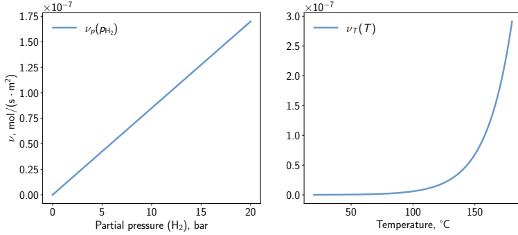
Figure 3.16: Trend of the developed correlation modeling the impact of (a) partial pressure ( T = 150^{\circ}\text{C} ) and (b) temperature ( p = 80\text{ bar} ) on the geochemical reaction
