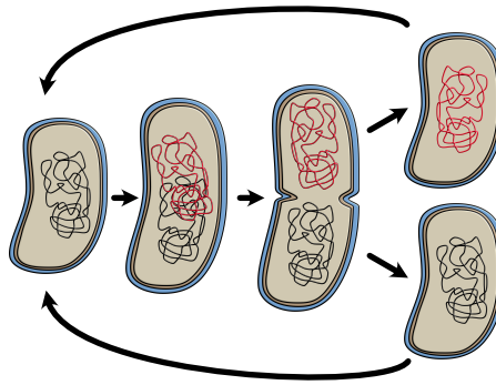
Figure 2.10: Schematic representation of cell division (binary fission)
