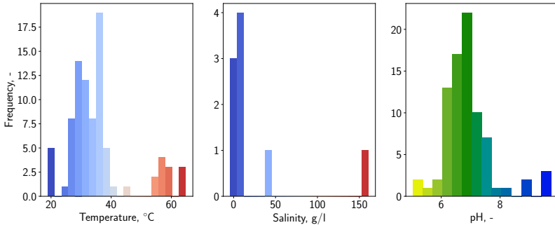
(C) Homoactogenic bacteria - \Delta T_v = 27^\circ\text{C} ; \Delta S_v = 43\text{ g/l} ; \Delta\text{pH}_v = 2.2
