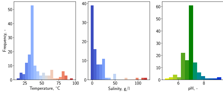
(A) Methanogenic archaea - \Delta T_v = 26^\circ\text{C} ; \Delta S_v = 69\text{ g/l} ; \Delta\text{pH}_v = 2.3
