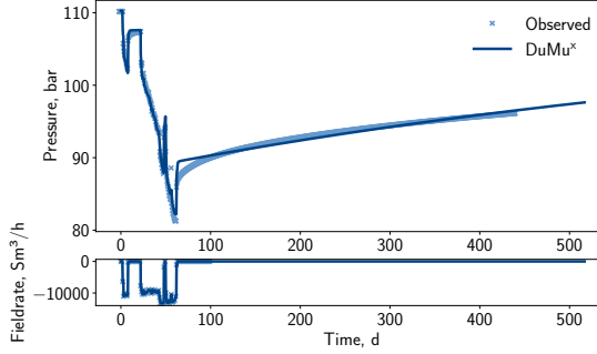
Figure 4.15: History match of the recent operation of the target formation including the observed and best match with DuMu x
