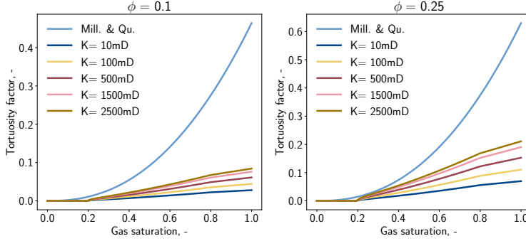
Figure 3.6: Comparison of tortuosity factor determined with Millington & Quirk and the proposed correlation as a function of gas saturation, porosity, and absolute permeability. To determine the impact of relative permeability, the Brooks-Corey model [18] is used, parameterized with S_{wc} = 0.2 and \lambda = 2
