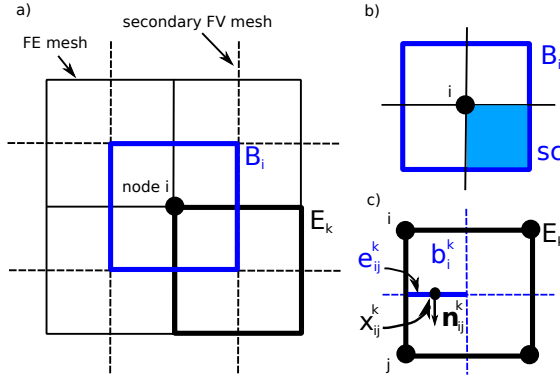
Figure 2.19: Overview of the different grids (a) and subgrids during the box method. (b) corresponds to the FV and (c) to FE mesh respectively [86]
