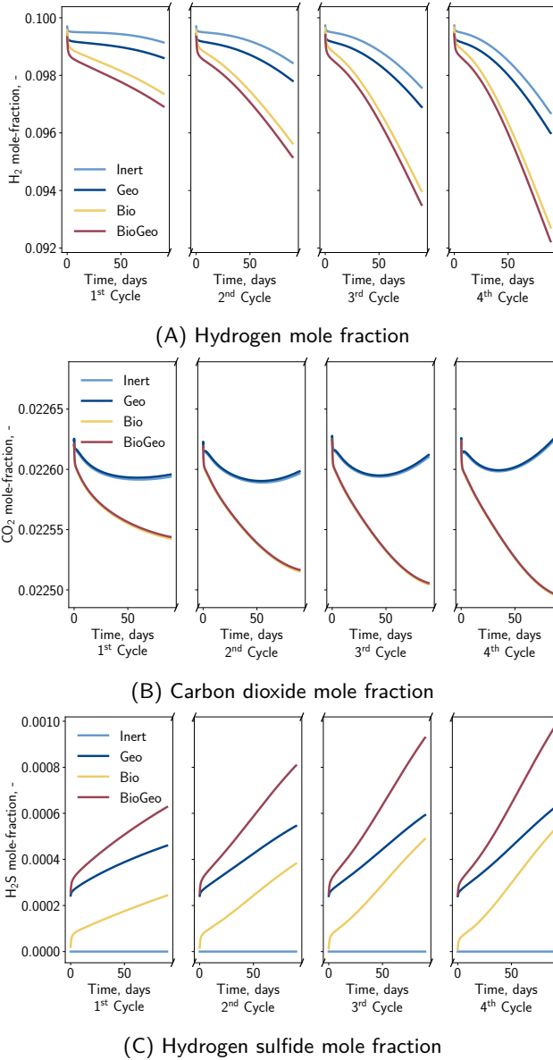
Figure 3.21: Gas composition in the gas stream during the four withdrawal phases
