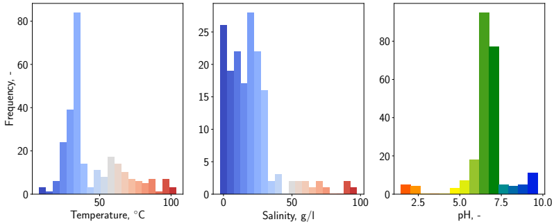
(B) Sulfate reducing bacteria - \Delta T_v = 24^\circ\text{C} ; \Delta S_v = 80\text{ g/l} ; \Delta\text{pH}_v = 2.5
