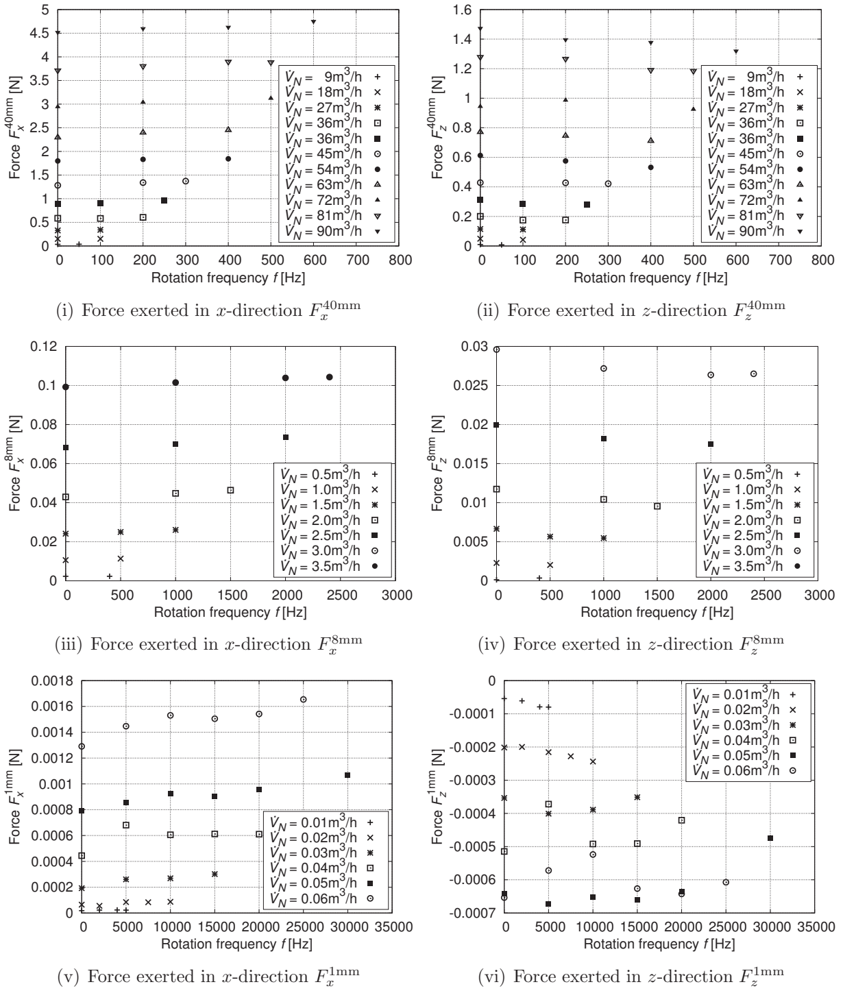
Figure 7.3: Forces F_x and F_z for all simulations conducted for 40 mm, 8 mm, and 1 mm
