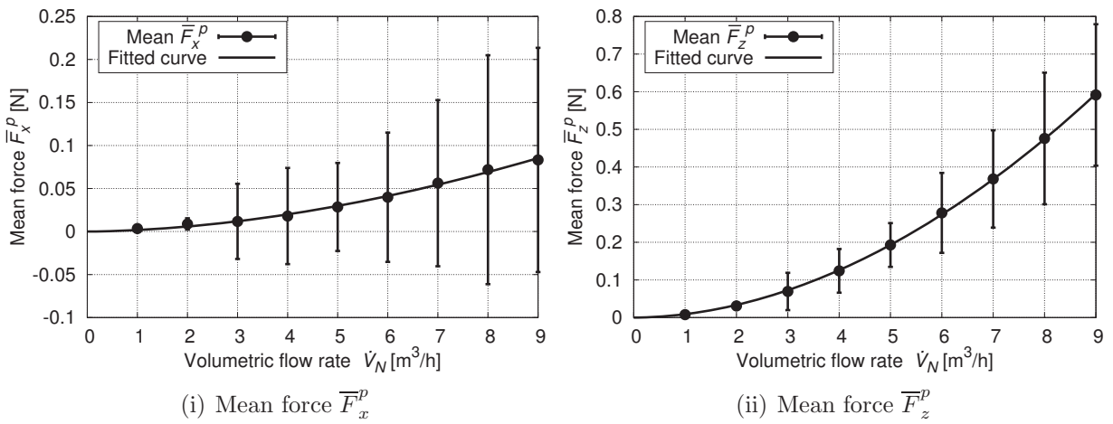
Figure 4.16: Mean forces \bar{F}_x^p and \bar{F}_z^p averaged over rotation frequency f for the prototype
