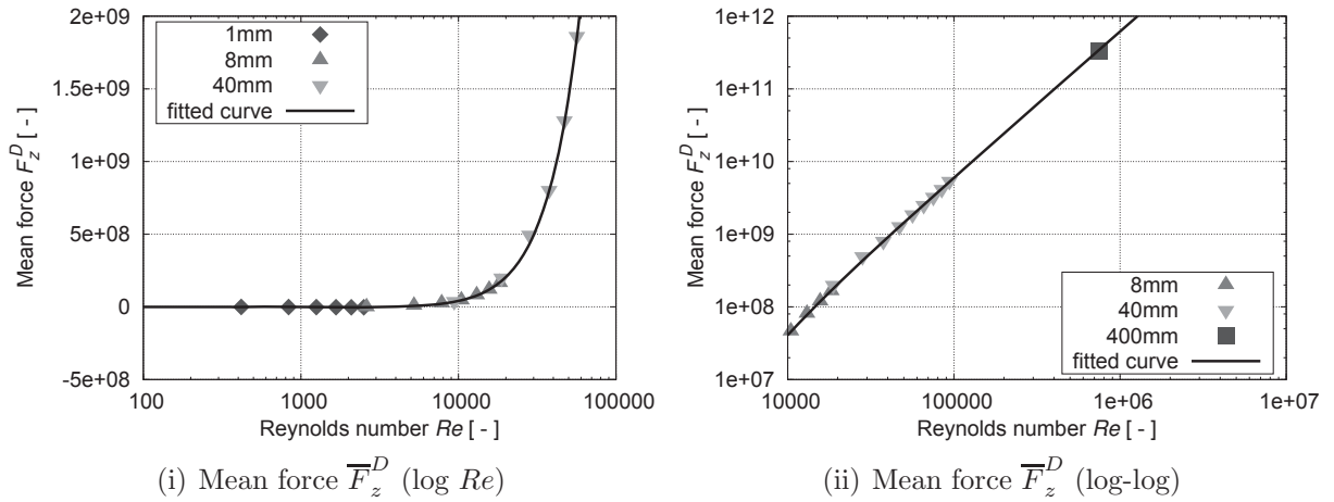
Figure 7.19: Mean force in z -direction \overline{F}_z^D over Reynolds number Re
