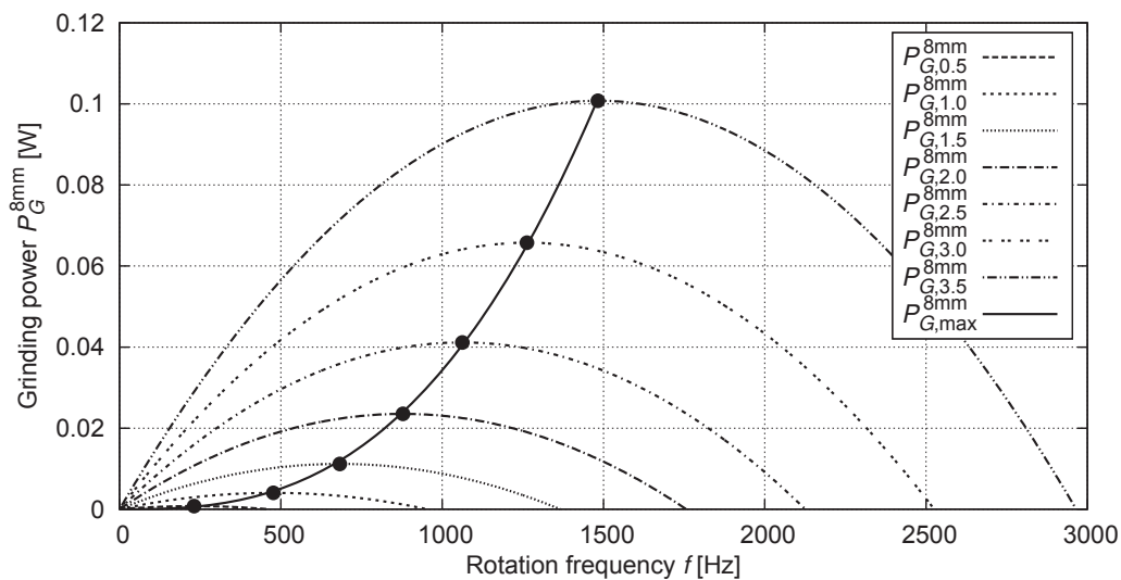
Figure 7.13: Grinding power P_G^{8\text{mm}} and P_{G,\max}^{8\text{mm}} for an 8 mm pneumatic sphere
