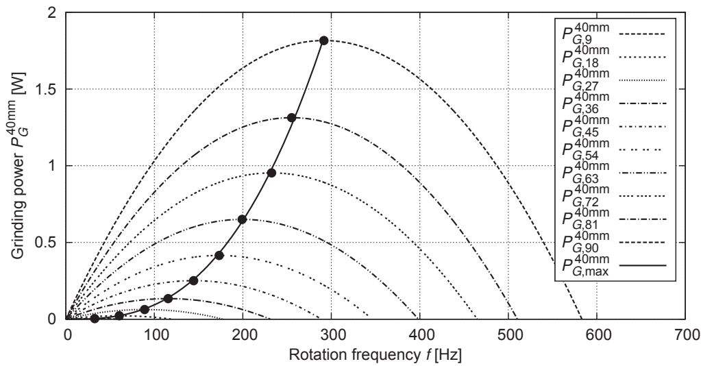
Figure 7.12: Grinding power P_G^{40\text{mm}} and P_{G,\max}^{40\text{mm}} for a 40 mm pneumatic sphere
