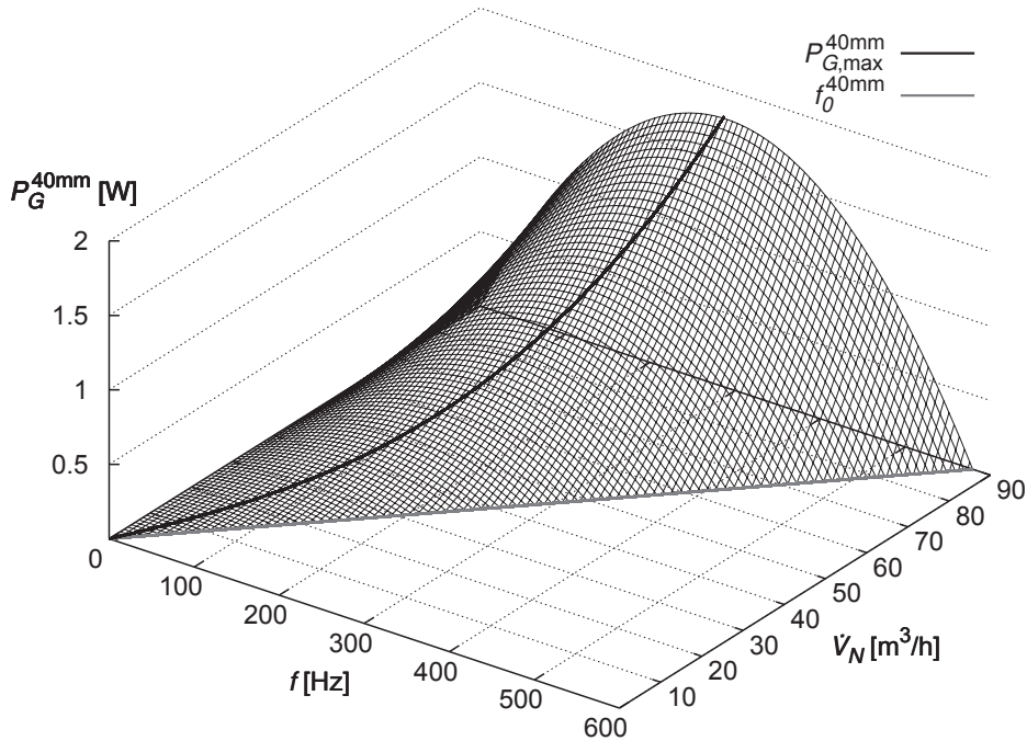
Figure 7.15: Grinding power P_G^{40\text{mm}} for a 40 mm pneumatic sphere
