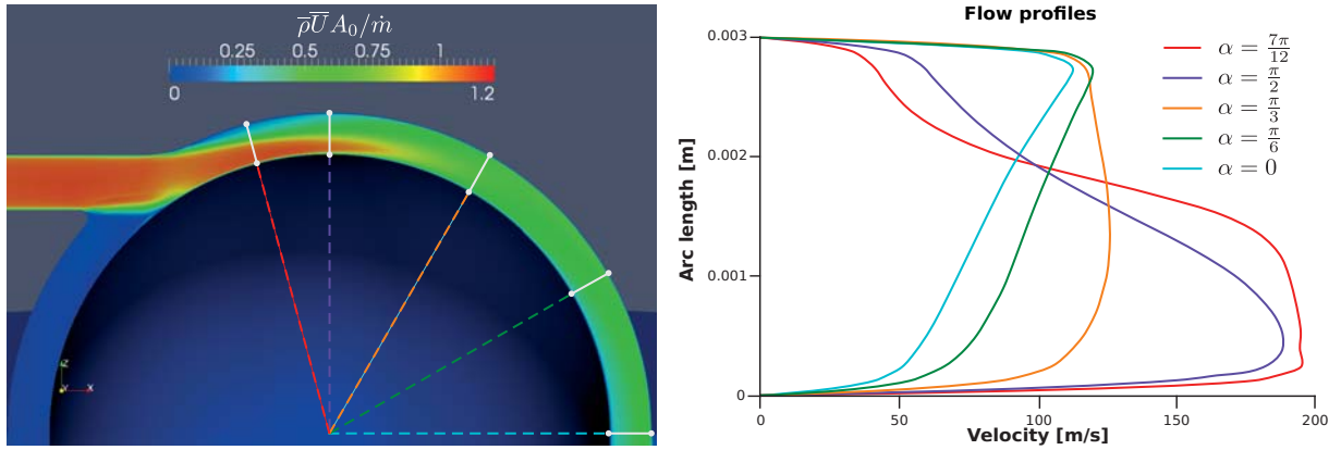
Figure 4.19: Flow profiles for f = 0 \text{ Hz} , \dot{V}_N = 8 \text{ m}^3\text{h}^{-1}
