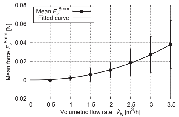
(iv) Mean force \overline{F}_z^{8\text{mm}}
