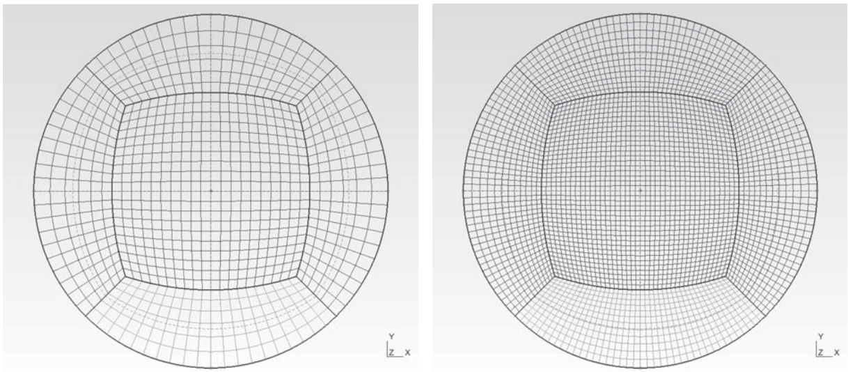
Figure B.3: Optimal butterfly mesh setup in coarse (left) and fine (right) variations
