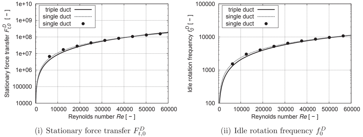
Figure 7.26: Stationary force transfer F_{t,0}^D and idle rotation frequency f_0^D over Reynolds number Re for single and triple duct geometries using air
