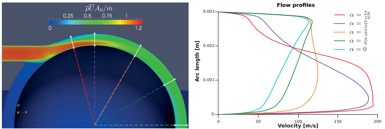
Figure 4.20: Flow profiles for f = 50 \text{ Hz} , \dot{V}_N = 8 \text{ m}^3\text{h}^{-1}
