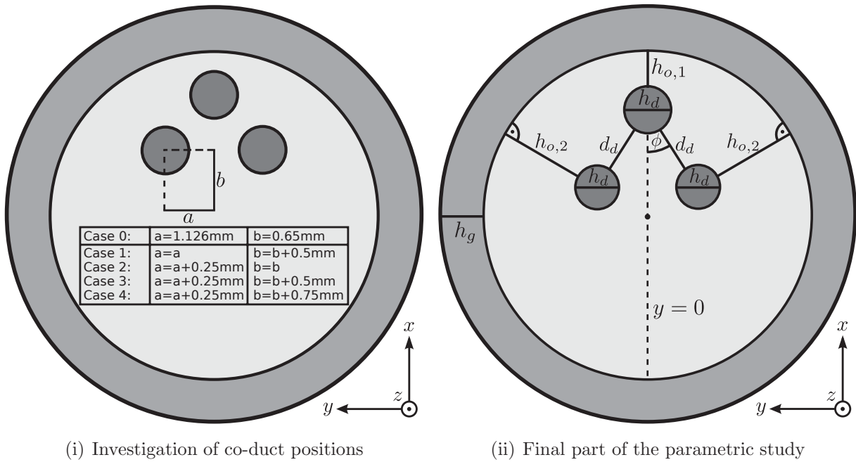
Figure 6.4: Further geometric parameters for the 8 mm GrindBall
