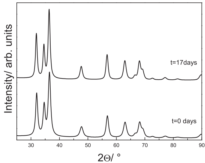
Figure 4.17: XRD pattern of ZnO nanoparticles before and after exposure to humid atmosphere. The Bragg reflections are getting narrower for the humidity exposed ZnO particles.
