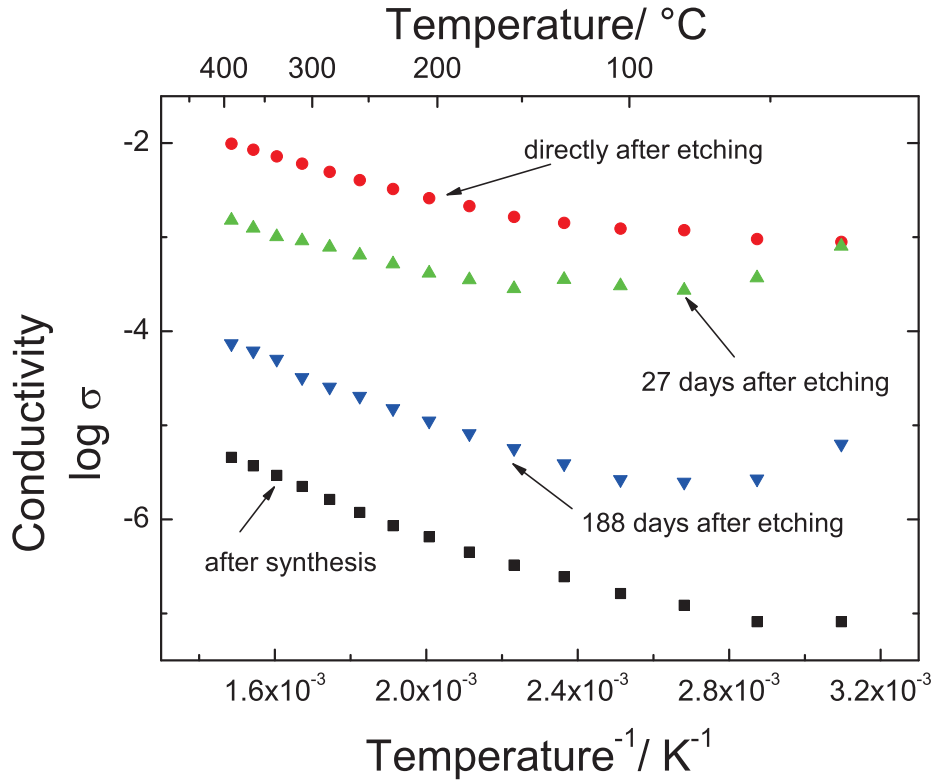
Figure 6.5: Conductivity for as-prepared and etched silicon nanoparticles as a function of the inverse temperature in hydrogen atmosphere.
