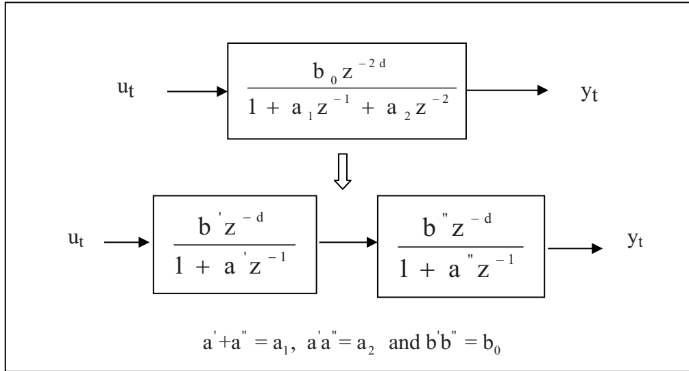
(b) Serial
