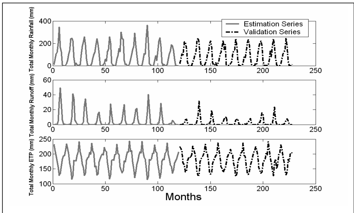
Figure 9.1vi Observed monthly rainfall, runoff and ETP for Debougou, Bourgouriba River (Black Volta Basin)
