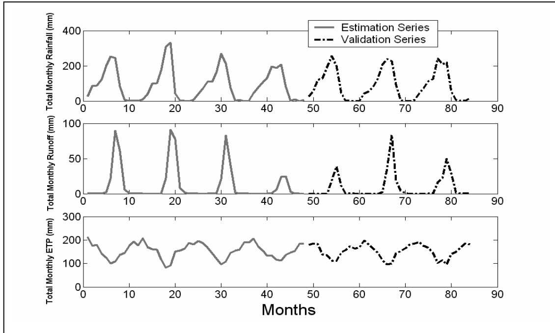
Figure 9.1xii Observed monthly rainfall, runoff and ETP for Nasia, Nasia River (White Volta Basin)
