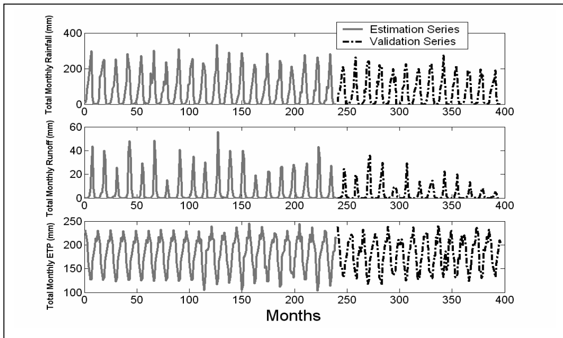
Figure 9.1xiv Observed monthly rainfall, runoff and ETP for Porga, Oti River
