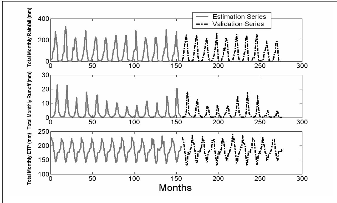
Figure 9.1vii Observed monthly rainfall, runoff and ETP for Lawra, Black Volta River
