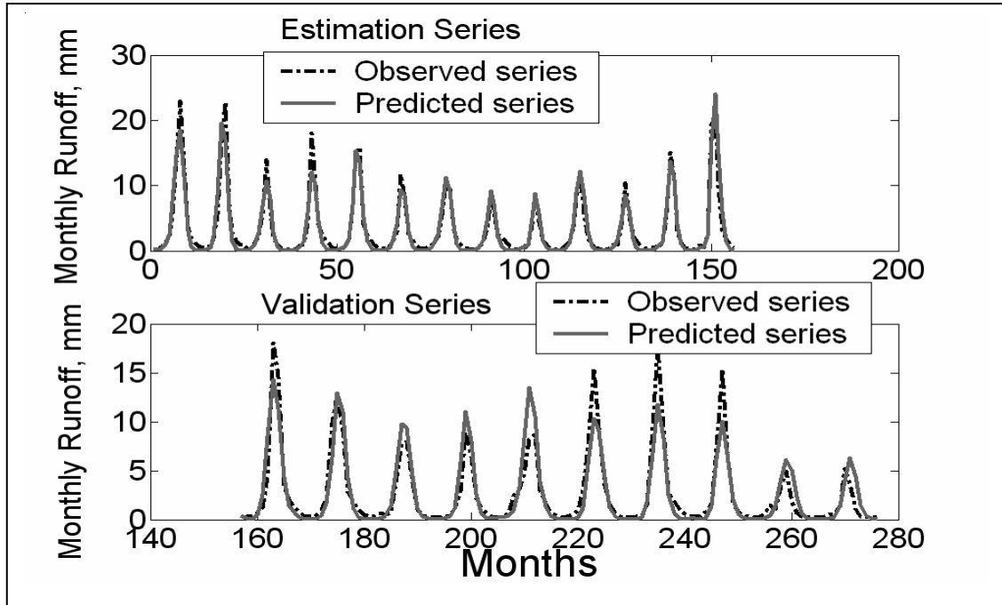
Figure 6.3 Observed and predicted monthly runoff for Lawra, Black Volta River LTI model [n \ m \ d] = [1 \ 2 \ 0]
