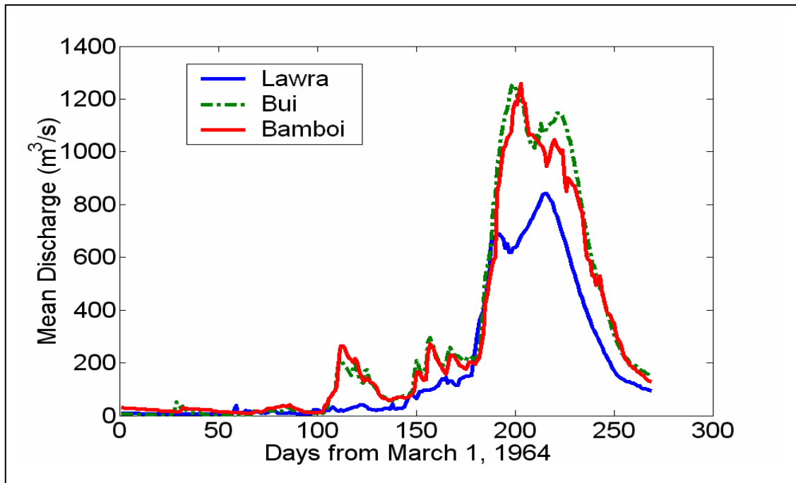
Figure 4.2a Daily hydrographs for stations Lawra, Bui and Bamboi on the Black Volta River (1964)
