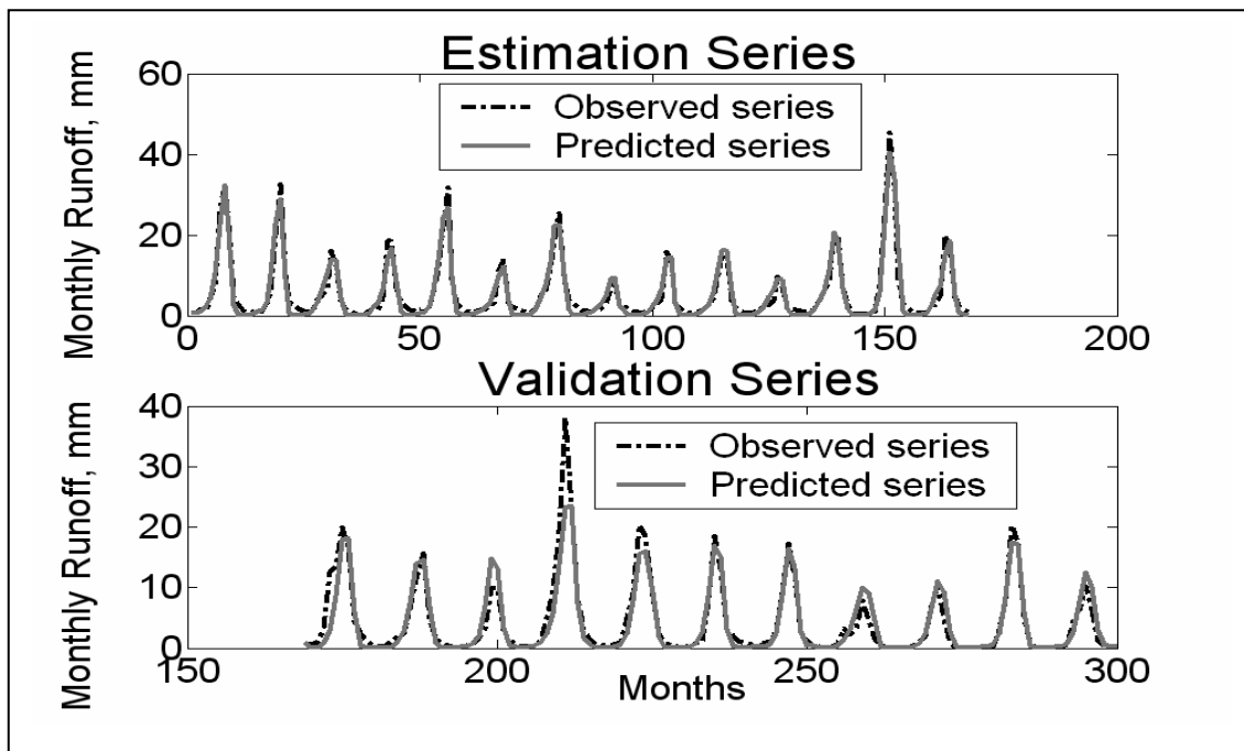
Figure 6.6 Observed and predicted monthly runoff for Bamboi, Black Volta River LTI model [n \ m \ d] = [1 \ 2 \ 0]
