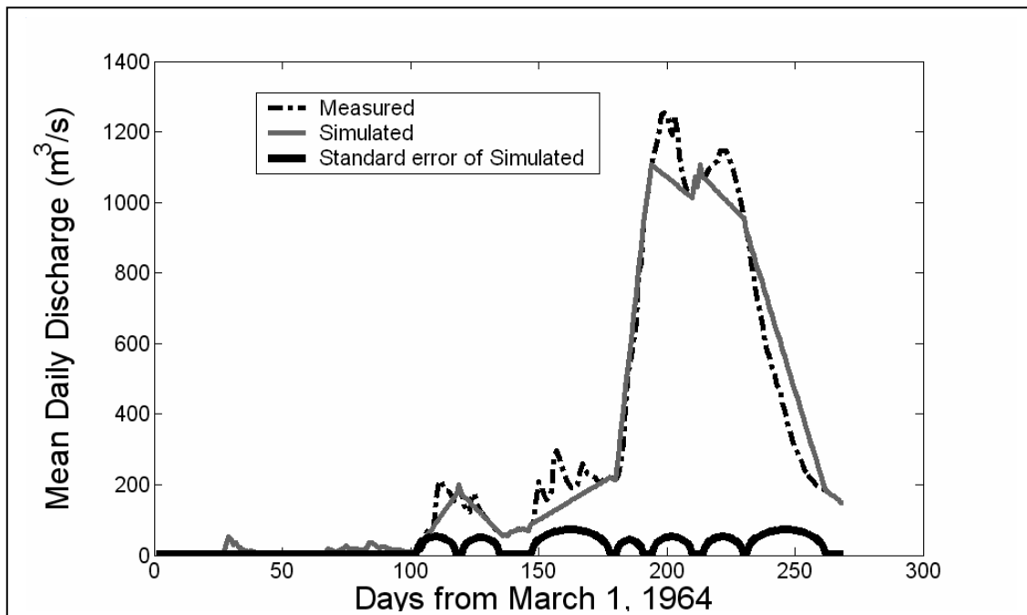
Figure 4.2b Measured and simulated daily hydrographs for station Bui on the Black Volta River; state space model on Bui discharge only (1964)
