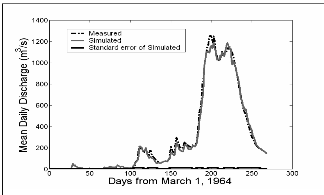
Figure 4.2c Measured and simulated daily hydrographs for station Bui on the Black Volta River; state space model on Bui, Lawra and Bamboi discharges (1964)
