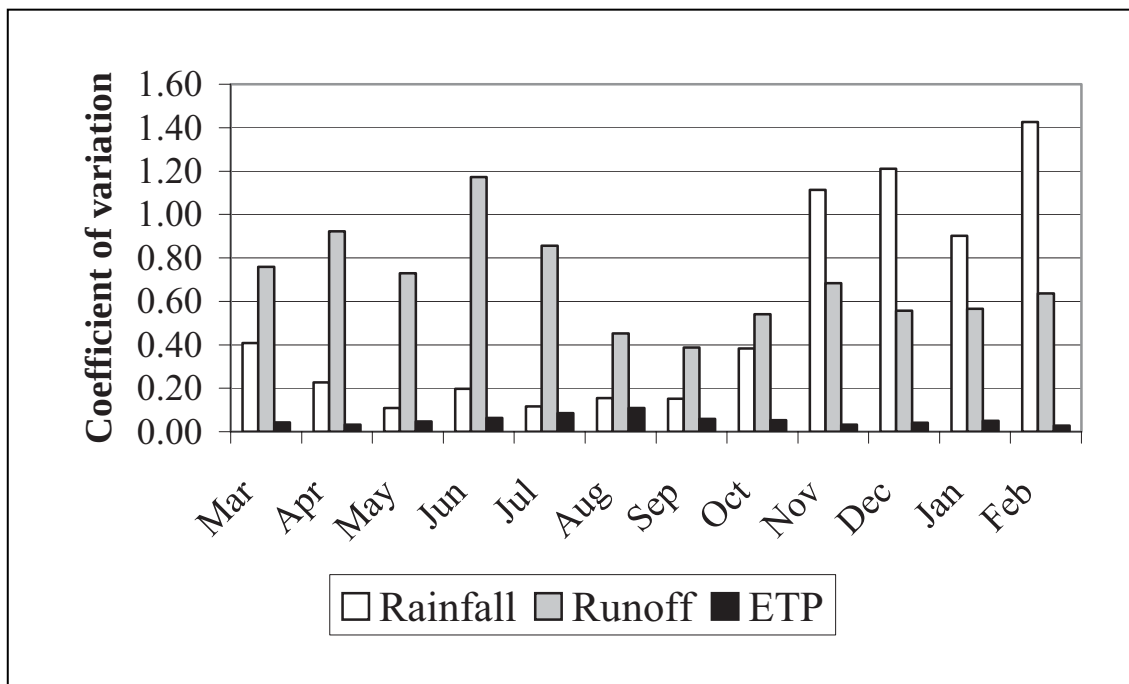
Figure 3.4d Coefficients of variation of monthly runoff, rainfall and potential evapotranspiration (ETP) at Sabari on the Oti River
