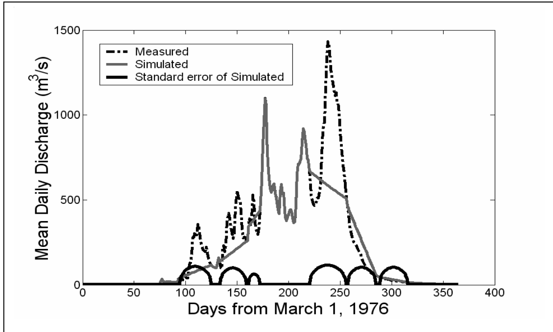
Figure 4.4b Measured and simulated daily hydrographs for Sabari on the Oti River; state space model on Sabari discharge only (1976)
