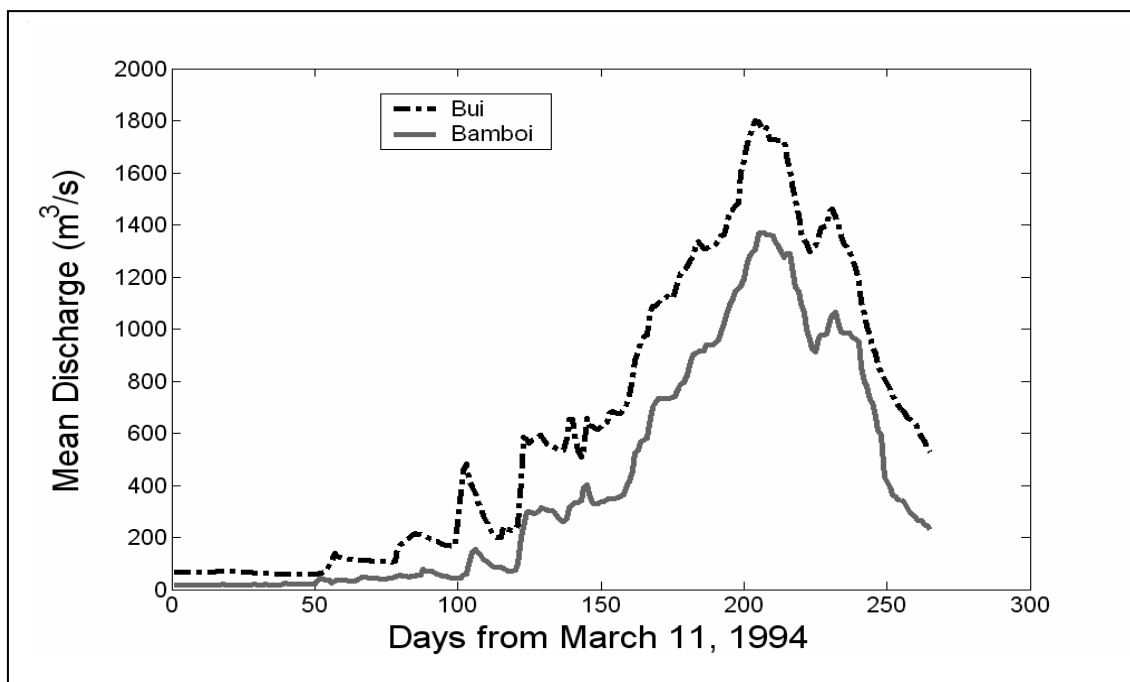
Figure 4.3a Daily hydrographs for Bui and Bamboi on the Black Volta River (1994)
