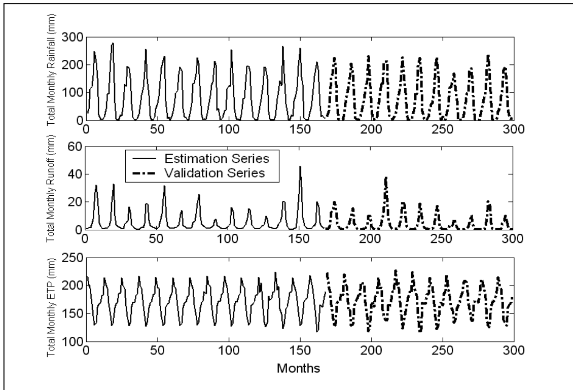
Figure 3.3a Observed monthly rainfall, runoff and ETP for Bamboi, Black Volta River
