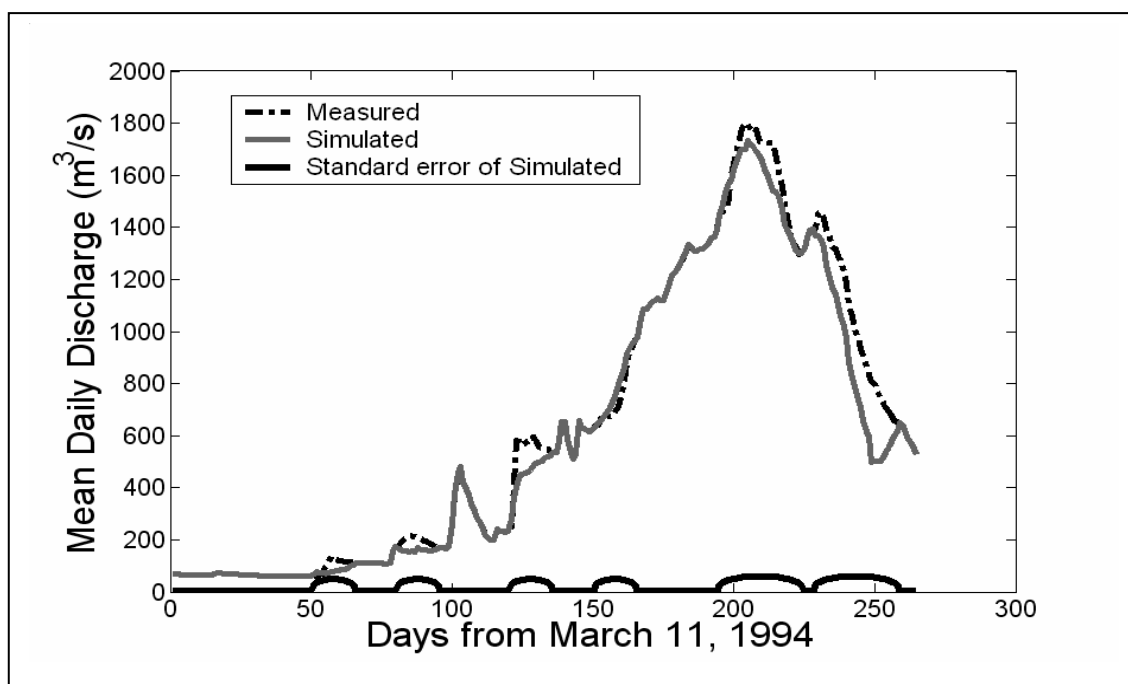
Figure 4.3c Measured and simulated daily hydrographs for Bui on the Black Volta River; state space model on Bui and Bamboi discharges (1994)
