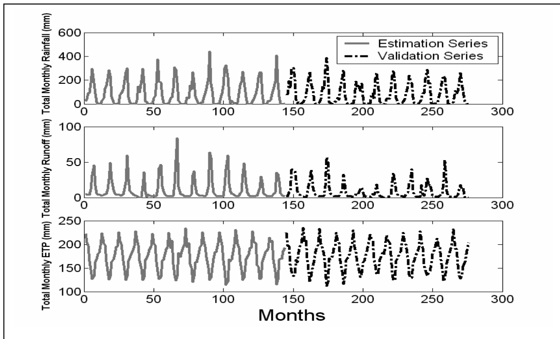
Figure 9.1i Observed monthly rainfall, runoff and ETP for Banzo, Black Volta River
