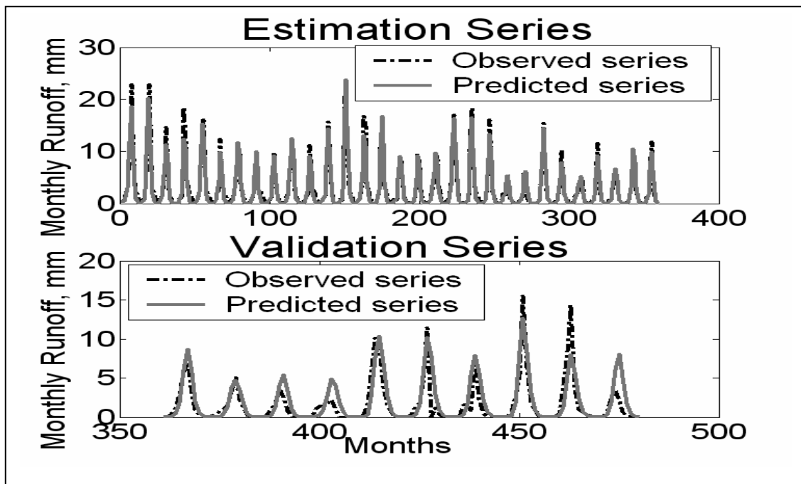
Figure 6.4 Observed and predicted monthly runoff for Dapola, Black Volta River LTI model [n \ m \ d] = [1 \ 2 \ 0]
