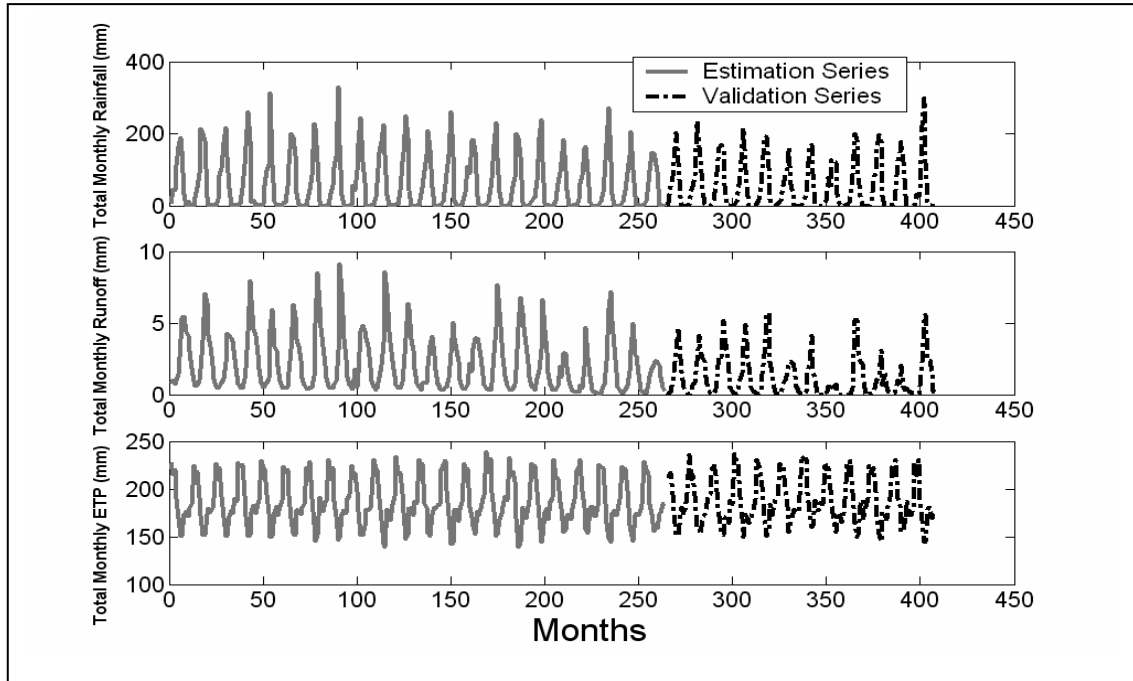
Figure 9.1v Observed monthly rainfall, runoff and ETP for Boromo, Black Volta River
