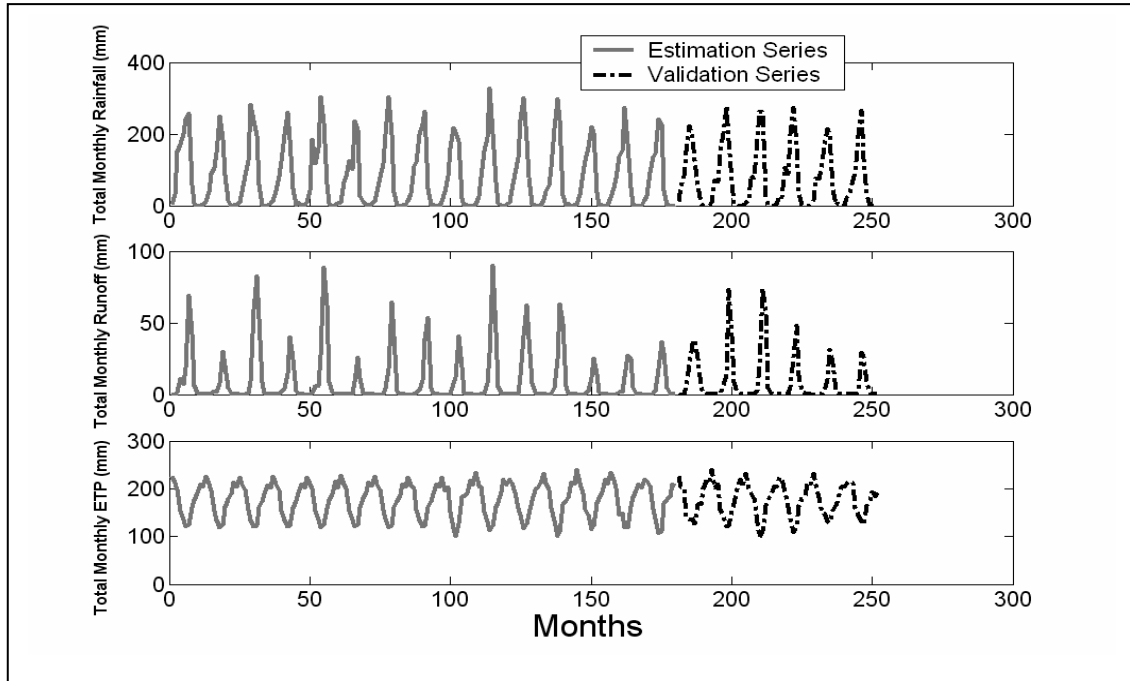
Figure 9.1xv Observed monthly rainfall, runoff and ETP for Mango, Oti River
