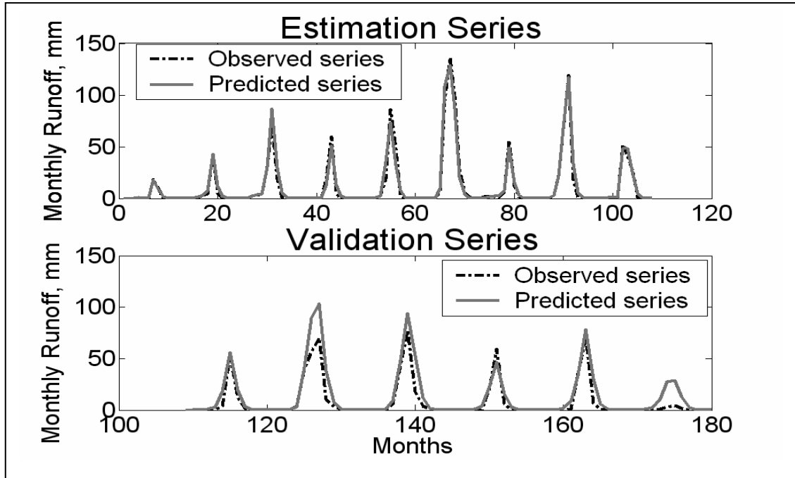
Figure 6.7 Observed and predicted monthly runoff for Yagaba, Kulpawn River (White Volta Basin) LTI model [n \ m \ d] = [1 \ 2 \ 0]
