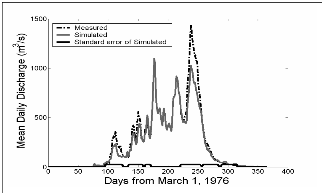
Figure 4.4c Measured and simulated daily hydrographs for Sabari on the Oti River; state space model on Sabari and Saboba discharges (1976)
