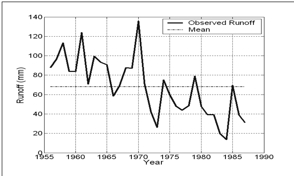
Figure 3.2a Annual hydrograph for Nwokuy on the Black Volta River
