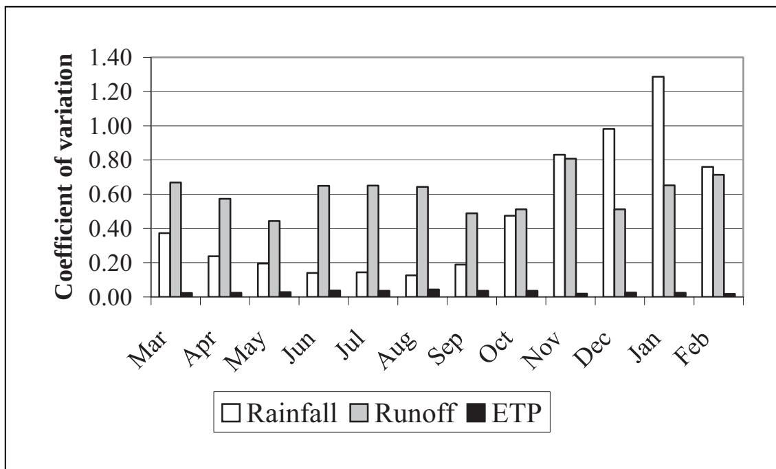
Figure 3.4b Coefficients of variation of monthly runoff, rainfall and potential evapotranspiration (ETP) at Bamboi on the Black Volta River
