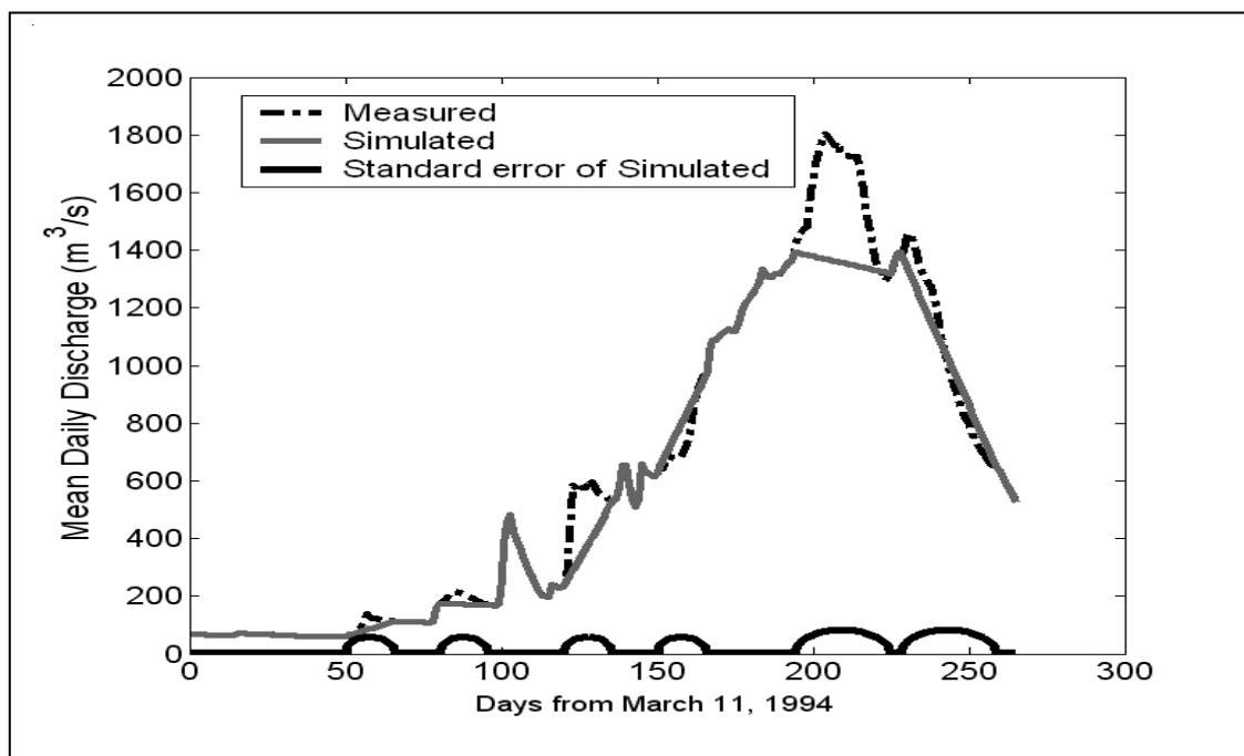
Figure 4.3b Measured and simulated daily hydrographs for Bui on the Black Volta River; state space model on Bui discharge only (1994)
