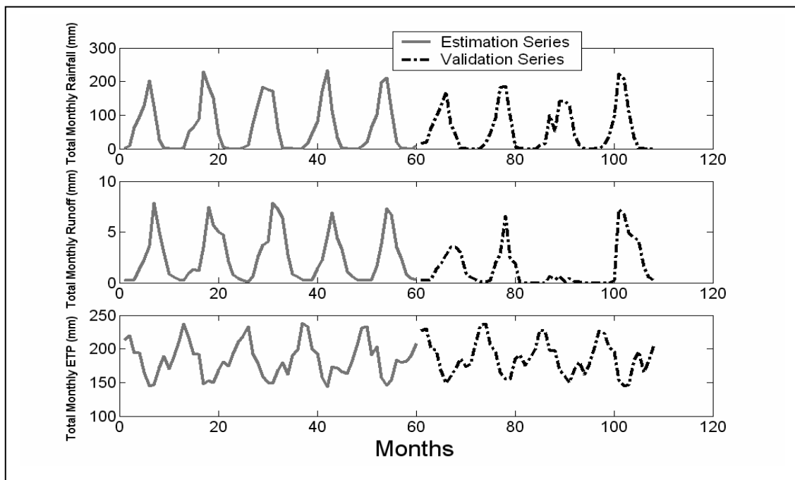
Figure 9.1iv Observed monthly rainfall, runoff and ETP for Tenado, Black Volta River
