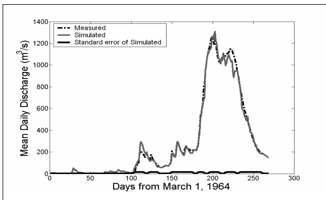
Figure 4.2d Measured and simulated daily hydrographs for Bui on the Black Volta River; state space model on Bui and Bamboi discharges (1964)
