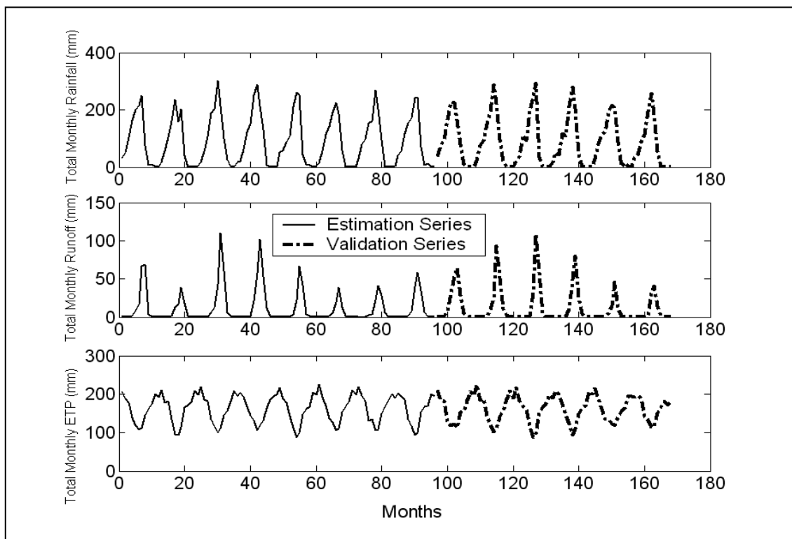
Figure 3.3b Observed monthly rainfall, runoff and ETP for Sabari, Oti River
