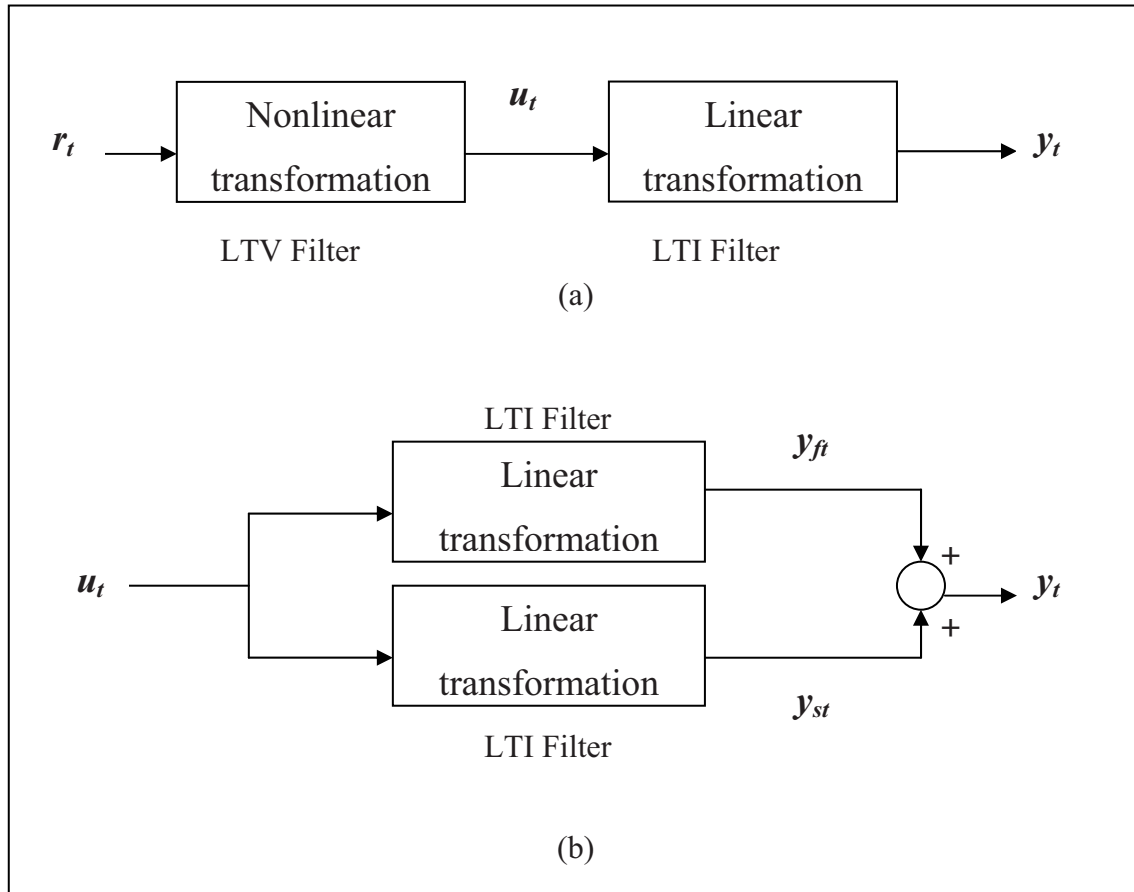
Figure 6.1 The rainfall-runoff transformation (a) Rainfall ( r_t ) \rightarrow Effective Rainfall ( u_t ) \rightarrow Total Runoff ( y_t ) transformations (b) Effective Rainfall transformations to two parallel flow components – Fast flow ( y_{ff} ) and Slow flow ( y_{sf} ) components
