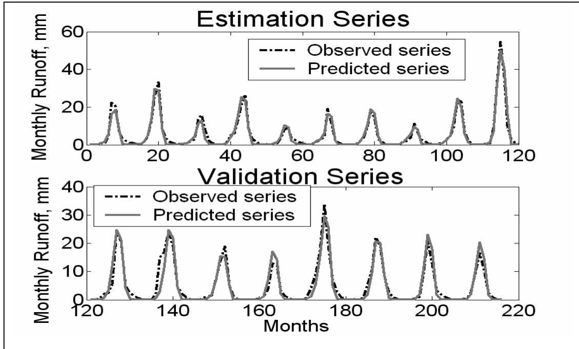
Figure 6.5 Observed and predicted monthly runoff for Bui, Black Volta River LTI model [n \ m \ d] = [0 \ 2 \ 0]
