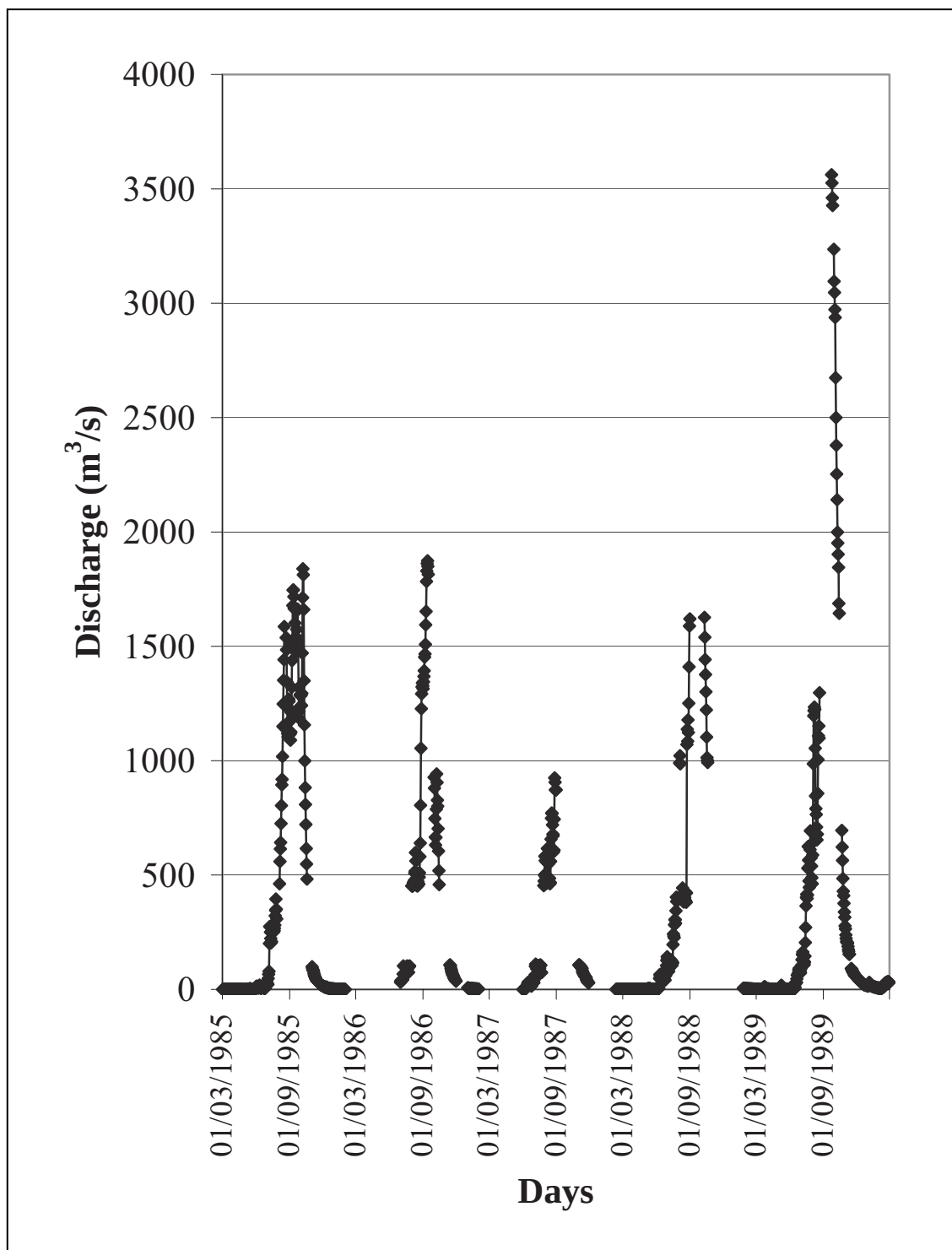
Figure 4.1 Daily hydrograph at Sabari on the Oti River (1985-1989). Typical pattern of gaps considered in the spatio-temporal modelling
