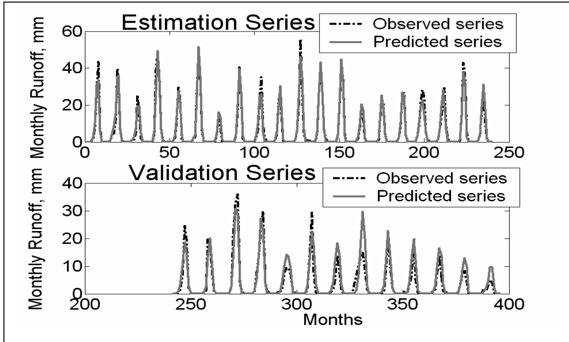
Figure 6.9 Observed and predicted monthly runoff for Porga, Oti River LTI model [n \ m \ d] = [1 \ 2 \ 0]
