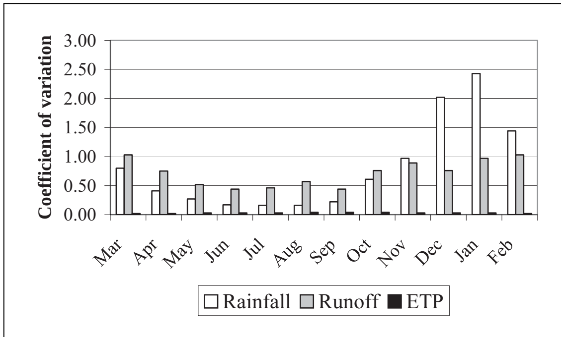
Figure 3.4a Coefficients of variation of monthly runoff, rainfall and potential evapotranspiration (ETP) at Dapola on the Black Volta River
