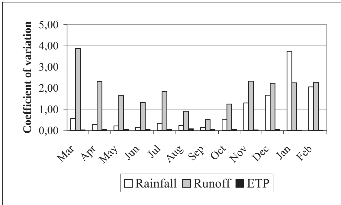
Figure 3.4c Coefficients of variation of monthly runoff, rainfall and potential evapotranspiration (ETP) at Yagaba on the Kulpawn River (White Volta Basin)
