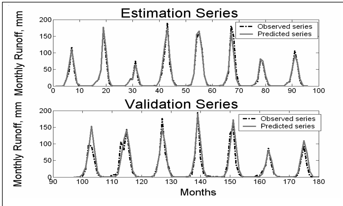
Figure 6.11 Observed and predicted monthly runoff for Koumangou, Koumangou River (Oti Basin) LTI model [n \ m \ d] = [1 \ 2 \ 0]
