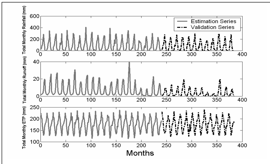
Figure 9.1ii Observed monthly rainfall, runoff and ETP for Nwokuy, Black Volta River
