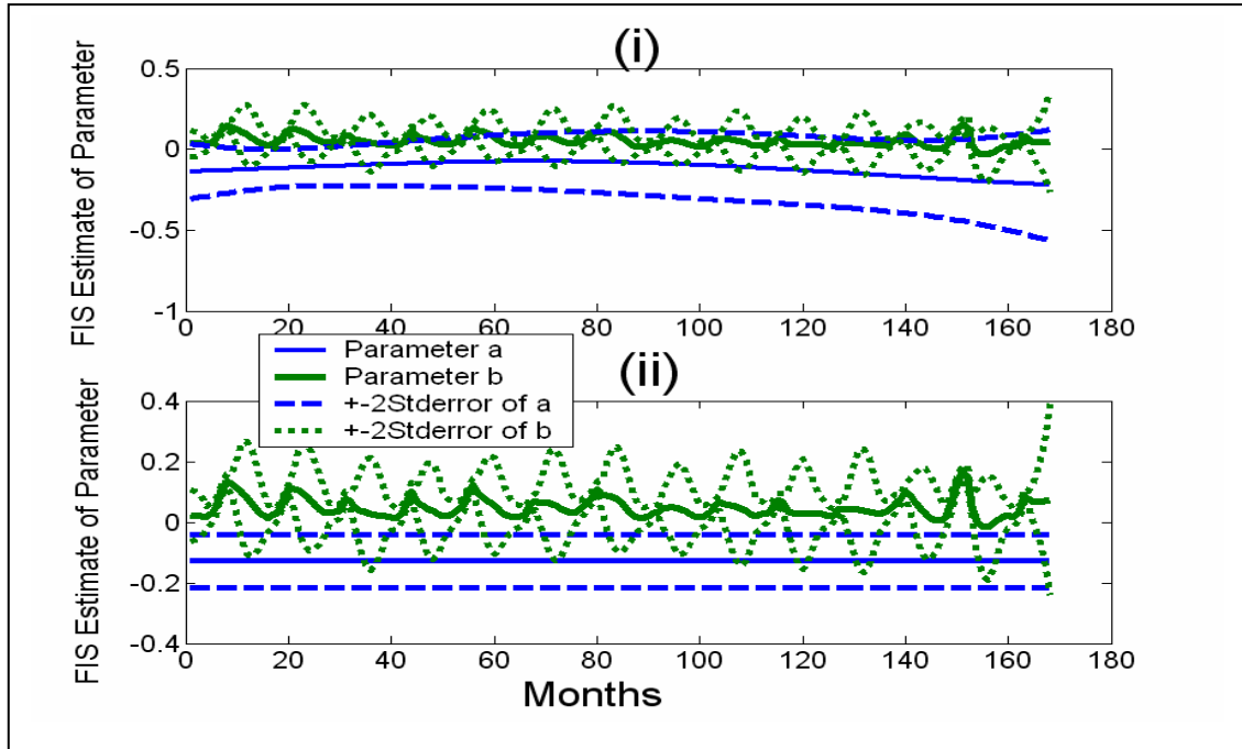
Figure 6.1 FIS estimated a and b parameters for Bamboi, Black Volta River (i) Both a and b state dependent (ii) Only b state dependent
