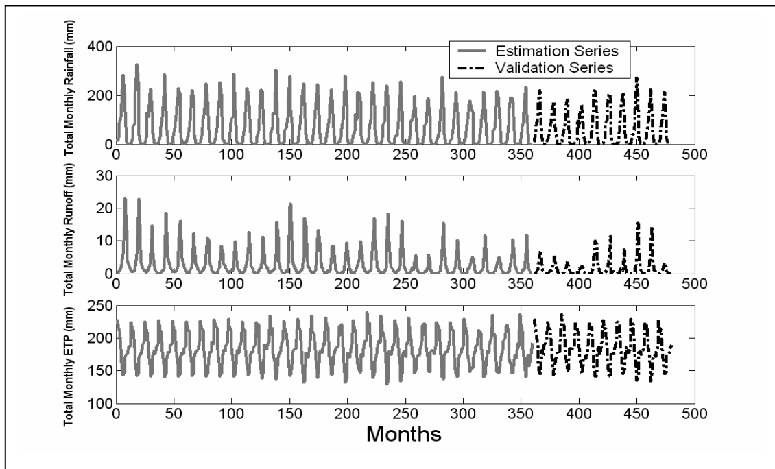
Figure 9.1viii Observed monthly rainfall, runoff and ETP for Dapola, Black Volta River
