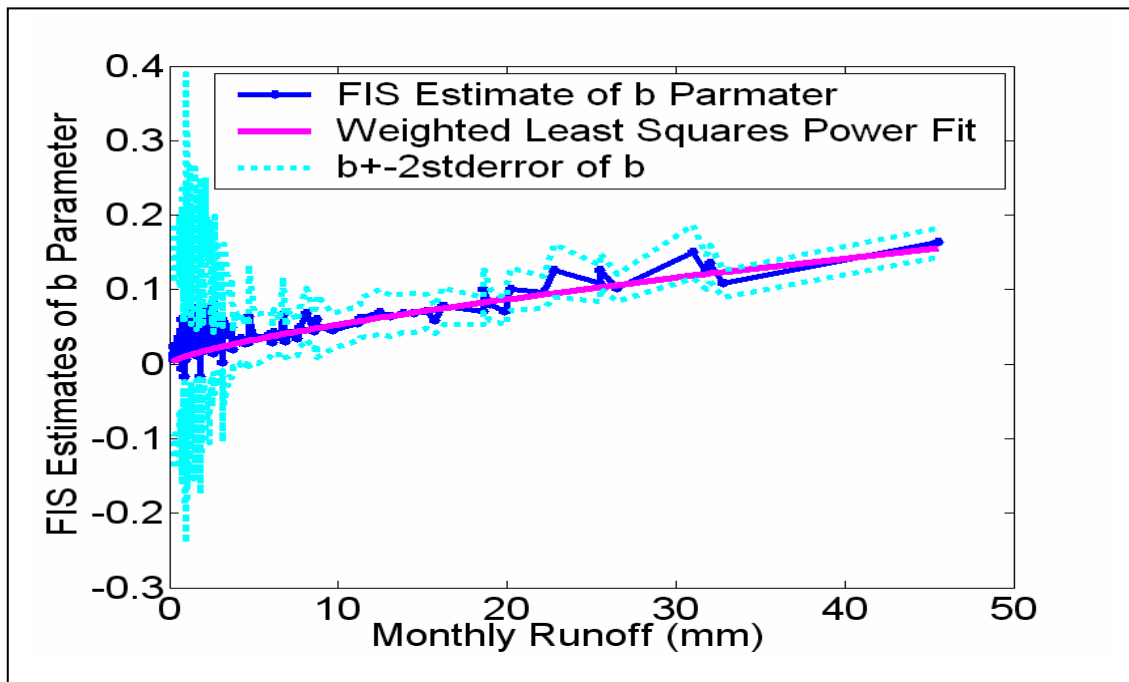
Figure 6.2 FIS estimates of the b parameter vs. monthly runoff for Bamboi, Black Volta River
