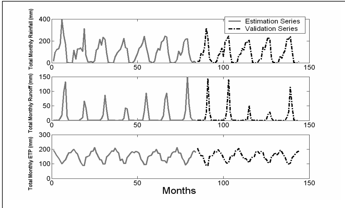
Figure 9.1xiii Observed monthly rainfall, runoff and ETP for Nabogo, Nabogo River (White Volta Basin)
