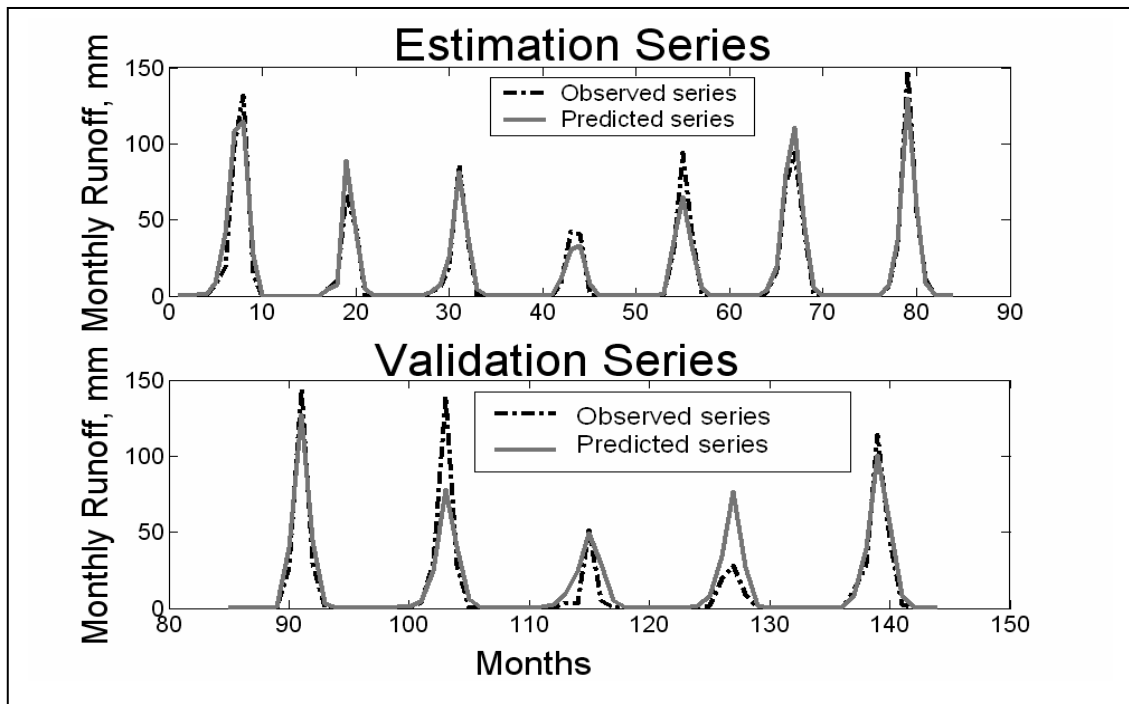
Figure 6.8 Observed and predicted monthly runoff for Nabogo, Nabogo River (White Volta Basin) LTI model [n \ m \ d] = [0 \ 2 \ 0]
