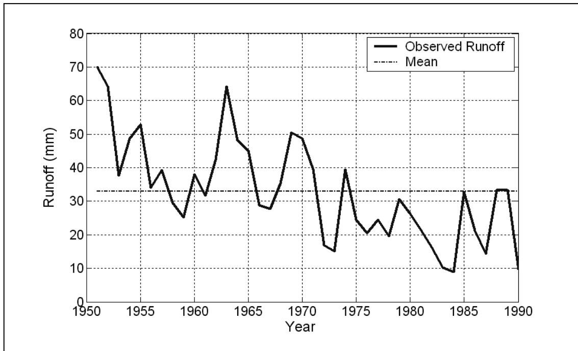
Figure 3.2c Annual hydrograph for Dapola on the Black Volta River
