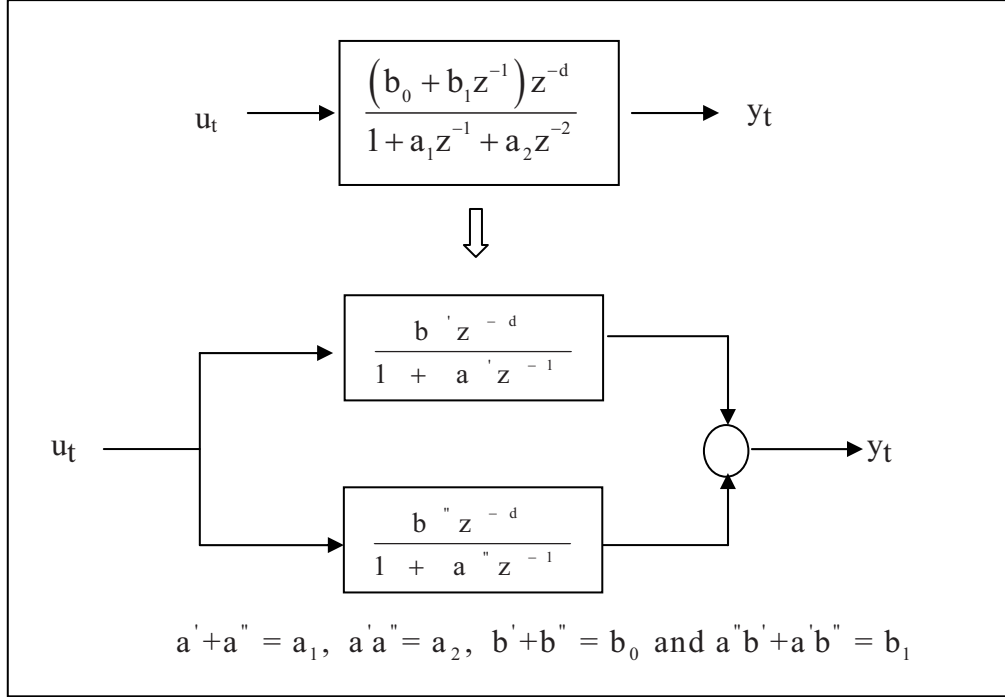
(a) Parallel
