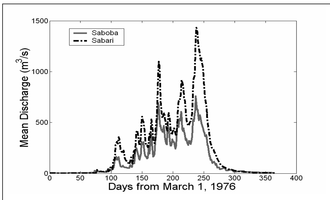
Figure 4.4a Daily hydrographs for Saboba and Sabari on the Oti River (1976)
