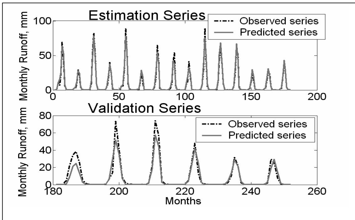
Figure 6.10 Observed and predicted monthly runoff for Mango, Oti River LTI model [n \ m \ d] = [0 \ 2 \ 0]
