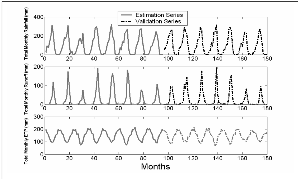
Figure 9.1xvi Observed monthly rainfall, runoff and ETP for Koumangou, Koumangou River (Oti Basin)
