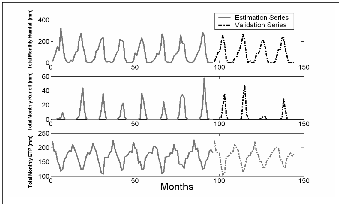
Figure 9.1x Observed monthly rainfall, runoff and ETP for Wiasi, Sisilli River (White Volta Basin)
