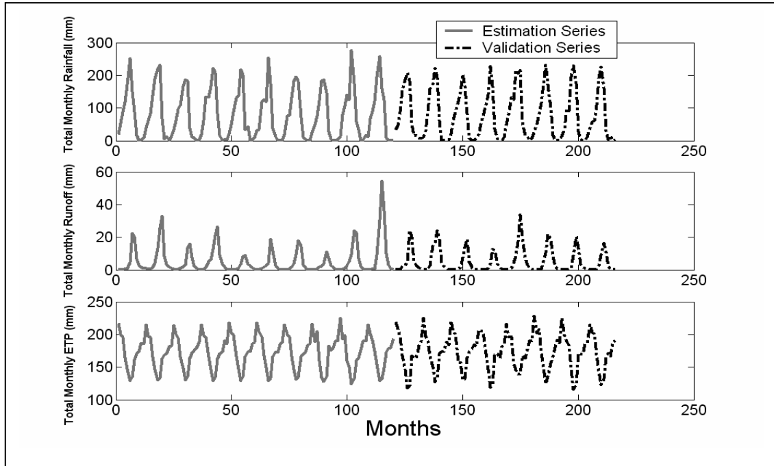
Figure 9.1ix Observed monthly rainfall, runoff and ETP for Bui, Black Volta River
