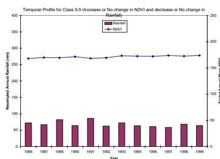
Figure 6.12 (cont.) Temporal profiles for the different classes of combinations
