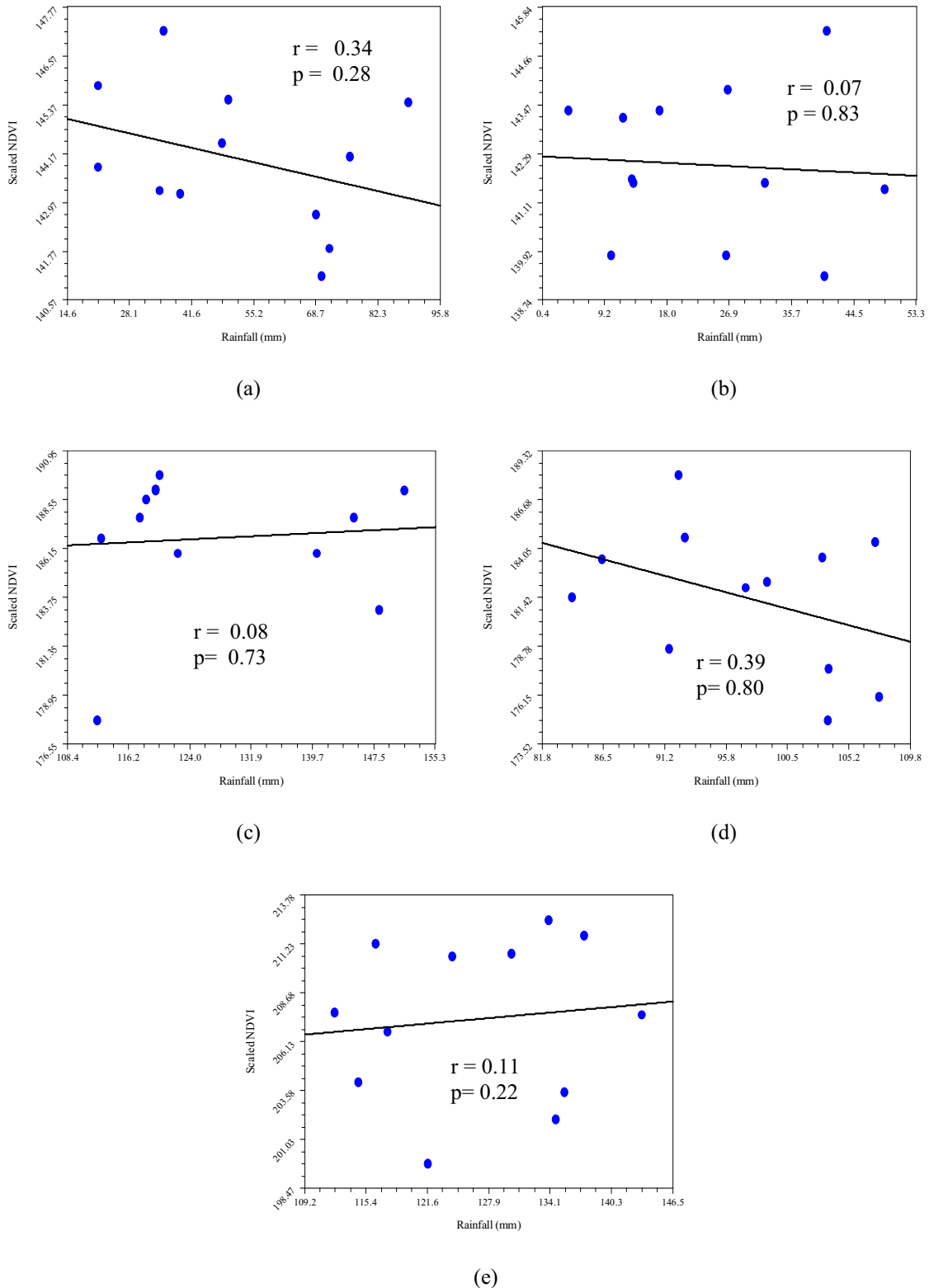
Figure 6.15 Correlation plots of NDVI and rainfall for the selected sites from changed areas of numerically comparable classes. Plot (a) represents the Sudan savanna site in north-west Nigeria from class 1:1, plot (b) represents the sahel site in the north-east of the country in class 2:2, plot (c) represents the forest site in the south-west of the country from class 3:3, plot (d) represents the site in the montane area around the central part of the country from class 4:4 and plot (e) represents the site in the humid dense forest in the south-east of the study area chosen from class 5:5. All these plots showed no significant correlation between NDVI and rainfall at p < 0.05 level. (Note that NDVI values as indicated were scaled from 0-255. To inter-convert, \text{scaled\_ndvi} = \text{float\_ndvi} \times 125 + 128 ).
