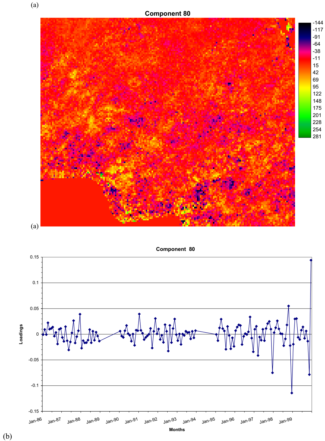
Figure 6.27. Component 80 Image and its loading graph. The component image is shown in (a) while its graph of loading scores is shown in (b). This is one of the last ‘low signal-to-noise ratio’ change component images. The image explains a very tiny proportion (0.057 %) of the total variance of the whole 144 monthly NDVI dataset, but exhibits an interesting change pattern. On the graph, the y – axis represents loading scores of the monthly NDVI image dataset and the x – axis represents their respective months.
